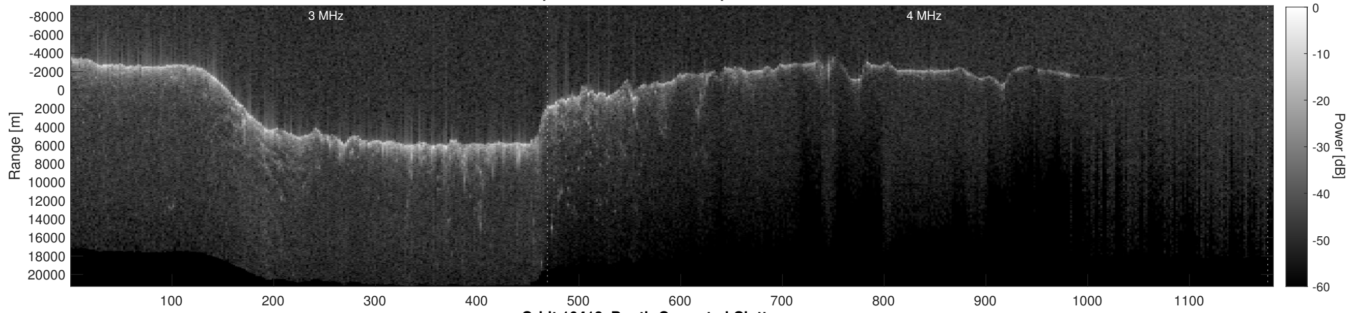
Orbit 10418, Depth-Corrected Cluttergram
