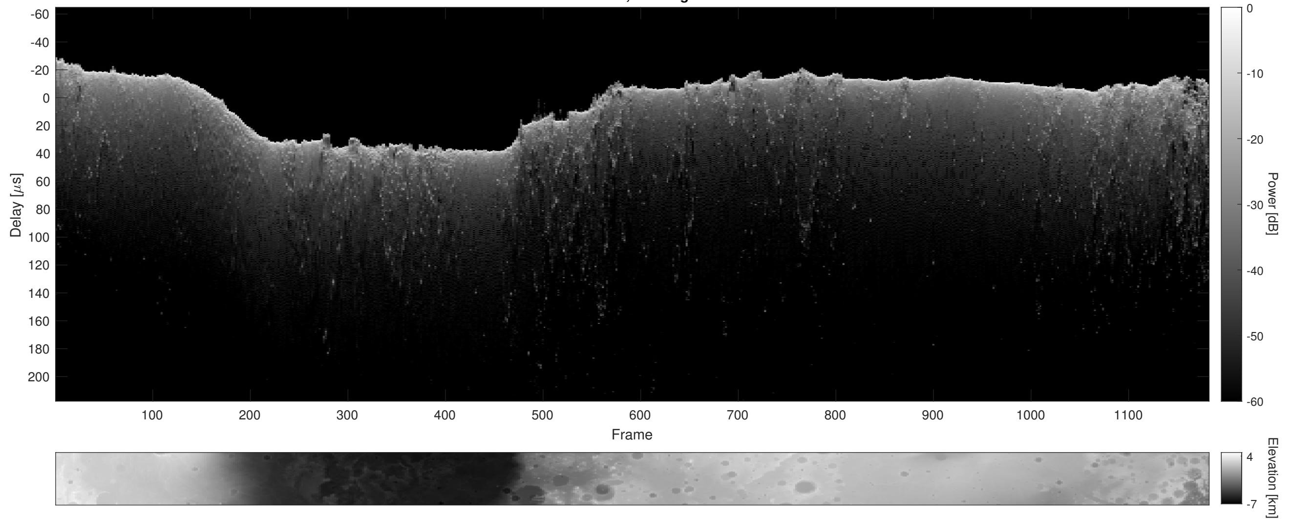
Orbit 10425, Cluttergram
