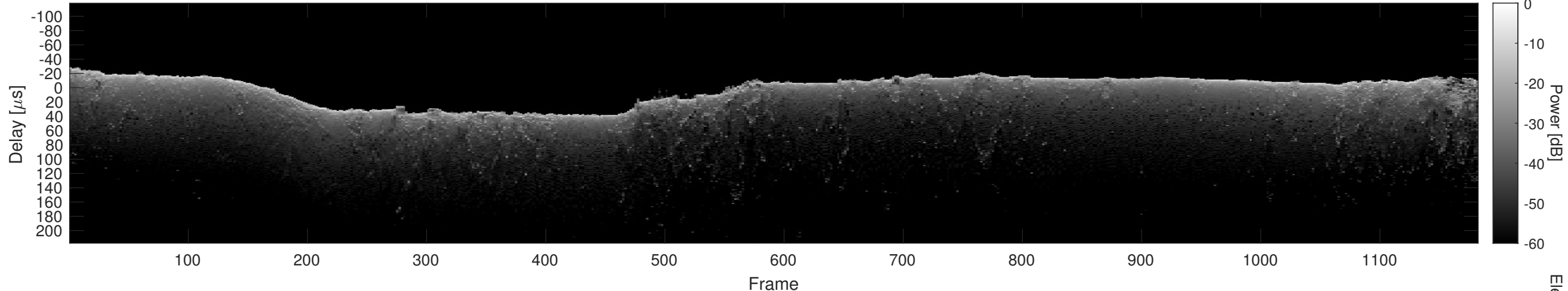
Orbit 10425, Cluttergram
