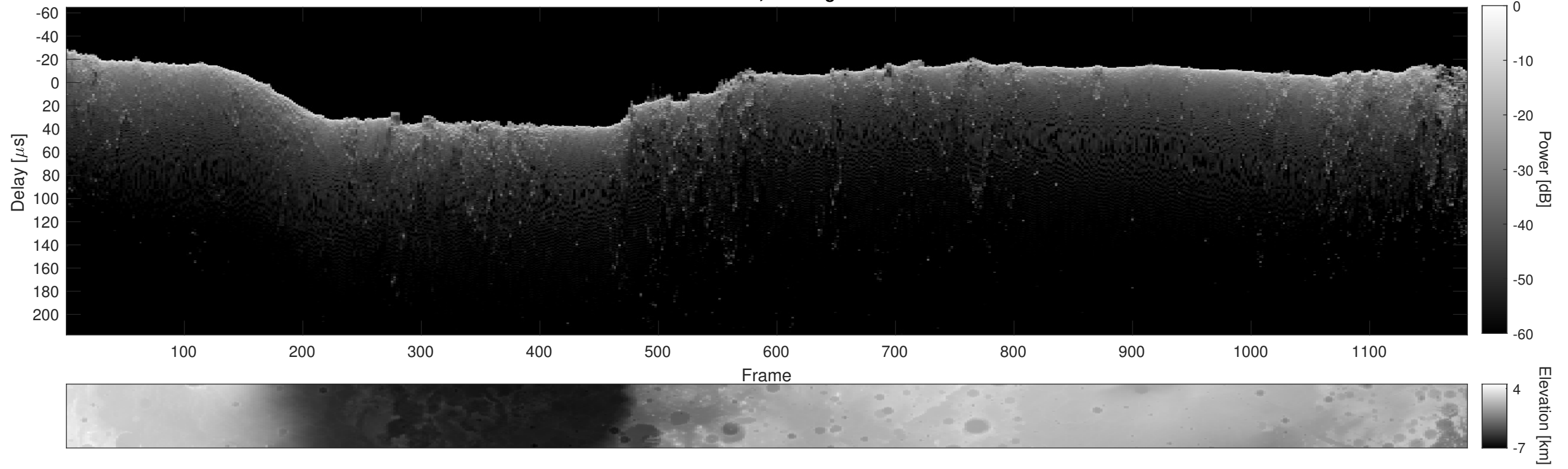
Orbit 10425, Cluttergram
