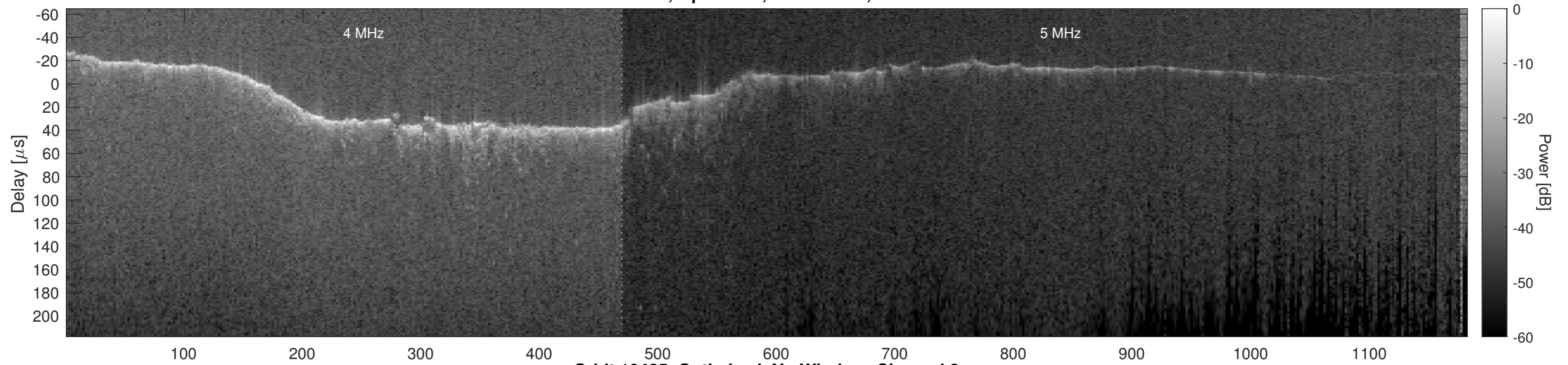
Orbit 10425, Optimized, No Window, Channel 2
