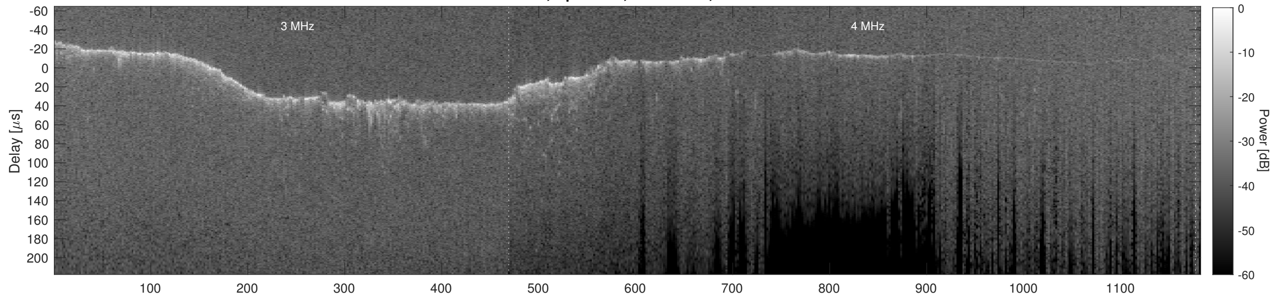
Orbit 10425, Cluttergram
