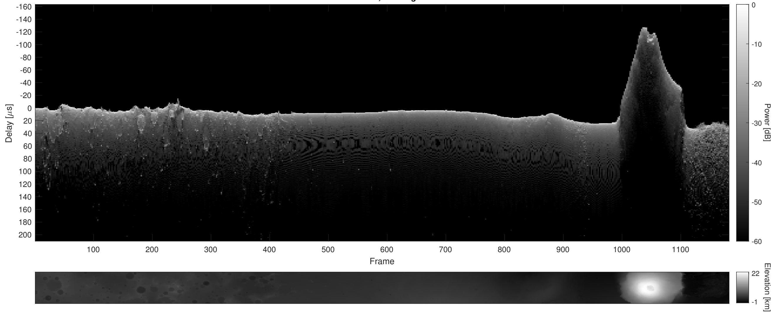
Orbit 10427, Cluttergram
