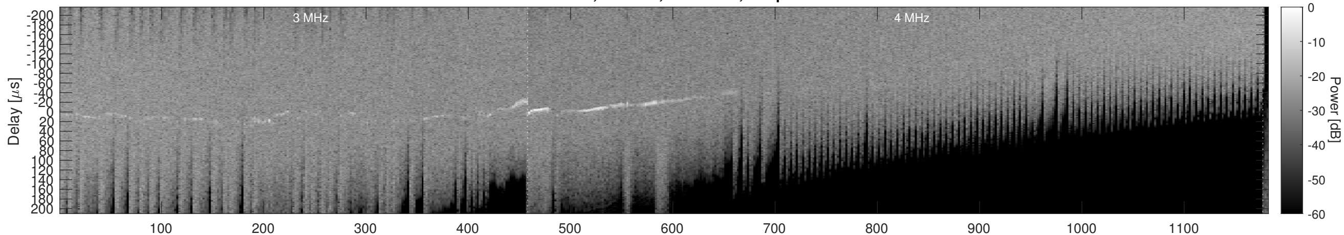
Orbit 10427, Window, Channel 2, Optimized
