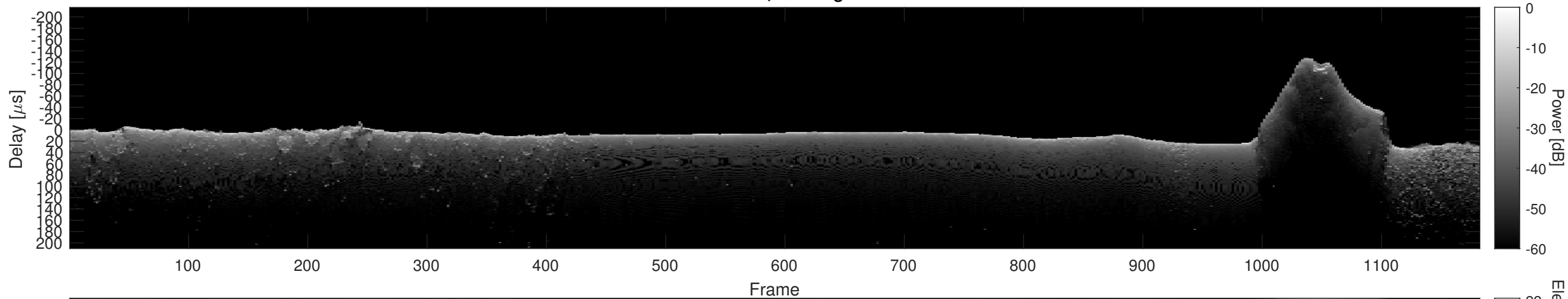
Orbit 10427, Cluttergram
