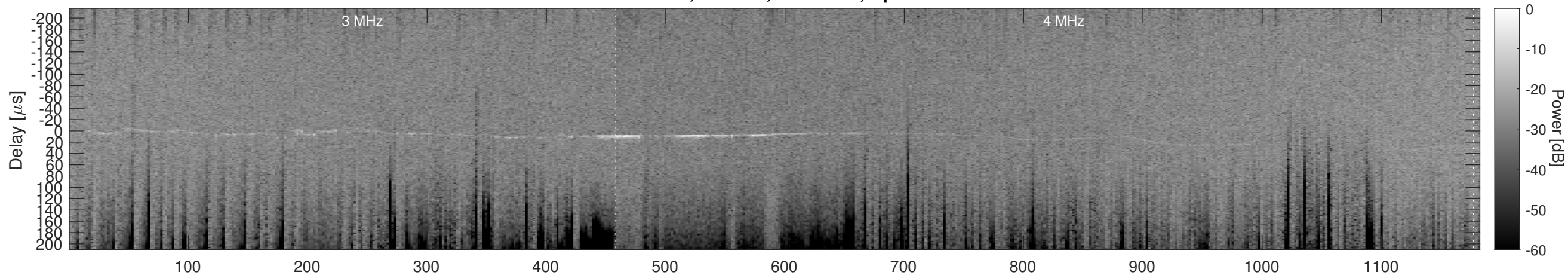
Orbit 10427, Cluttergram
