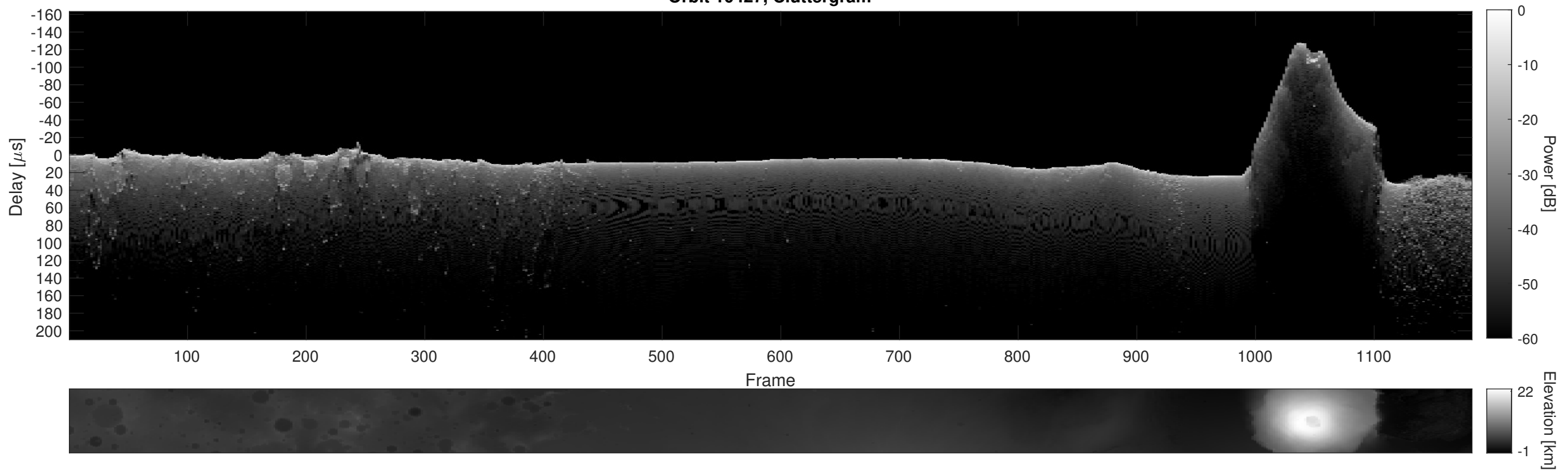
Orbit 10427, Cluttergram
