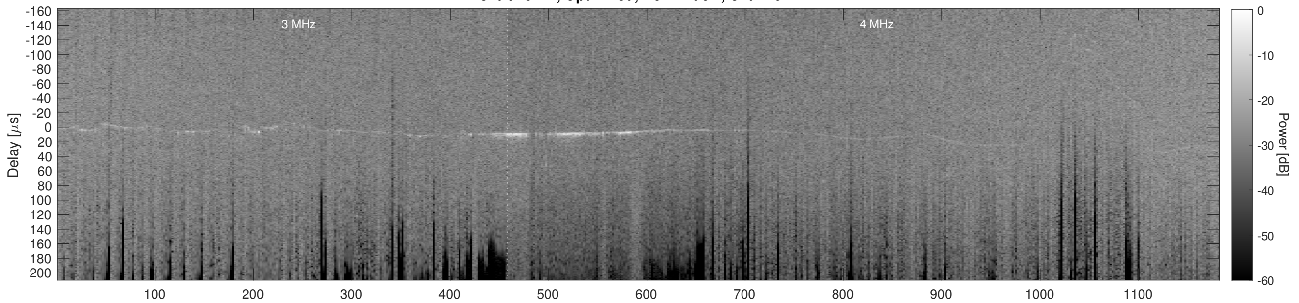
Orbit 10427, Cluttergram
