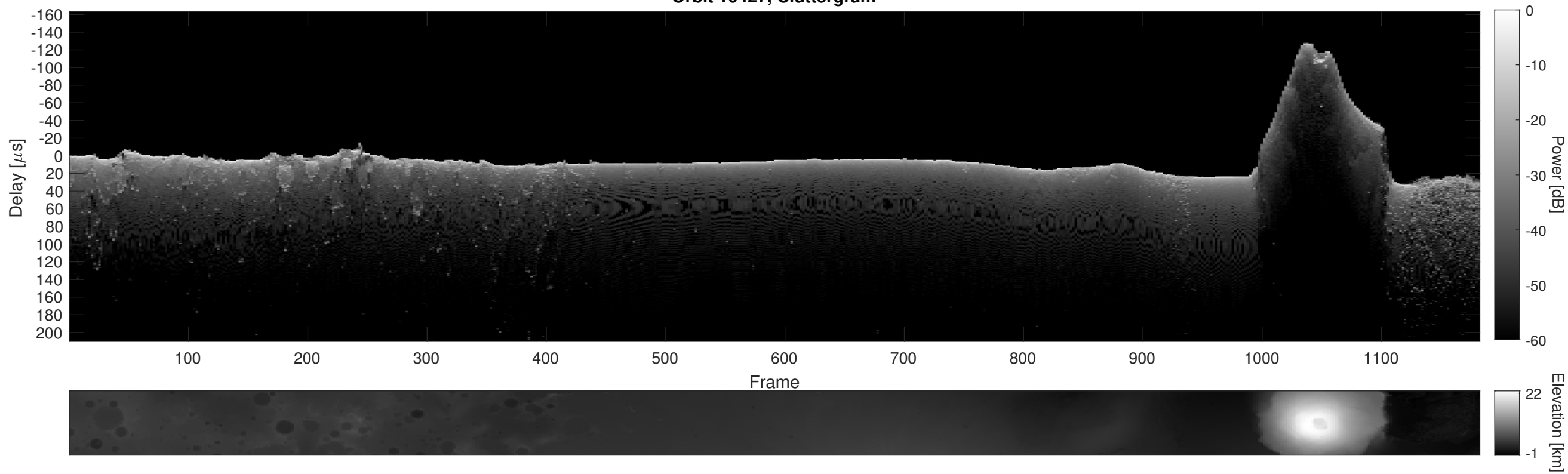
Orbit 10427, Cluttergram
