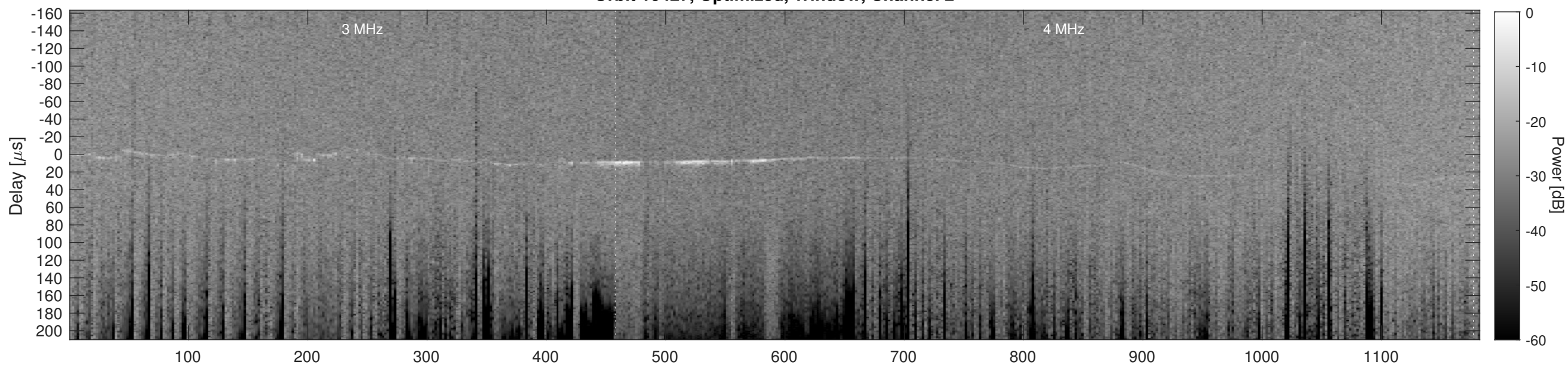
Orbit 10427, Cluttergram
