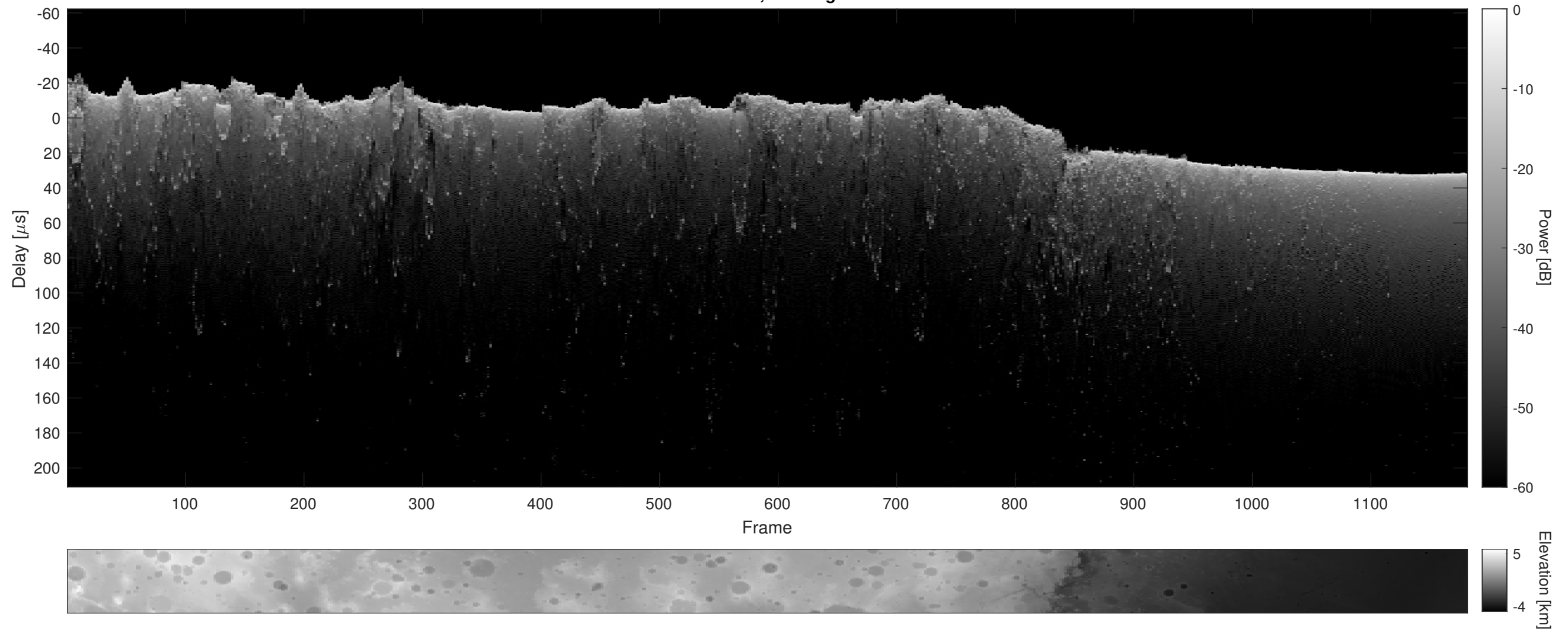
Orbit 10428, Cluttergram
