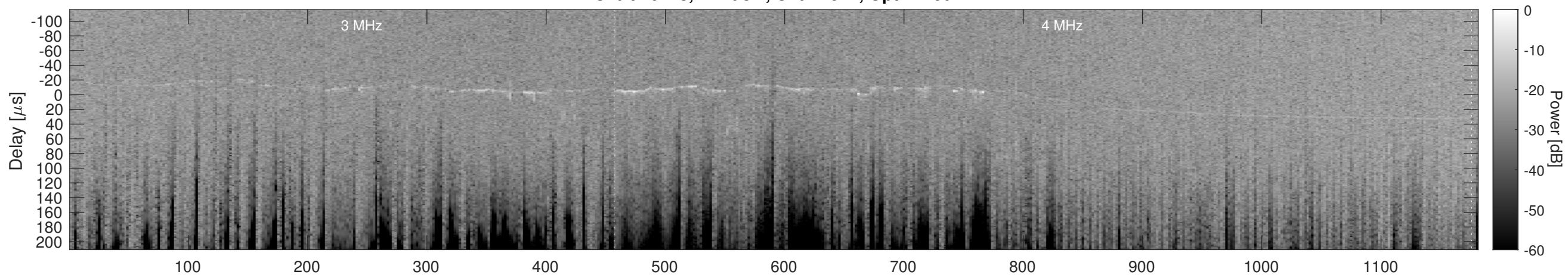
Orbit 10428, Cluttergram
