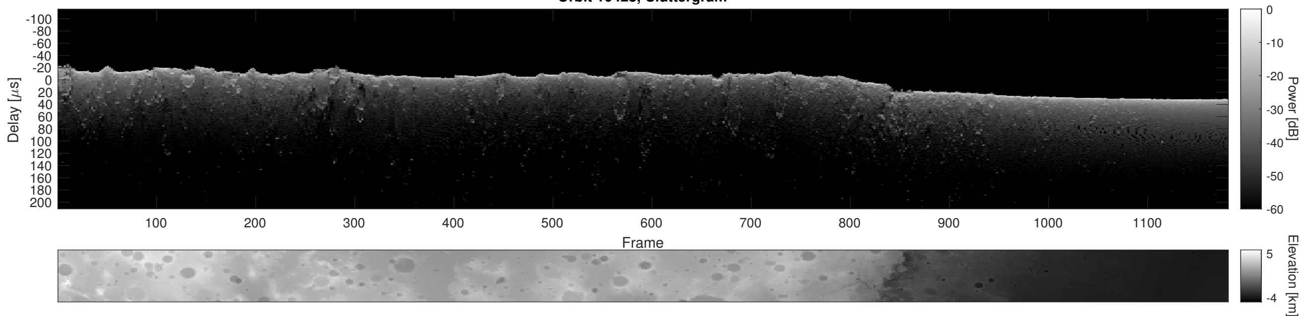
Orbit 10428, Cluttergram
