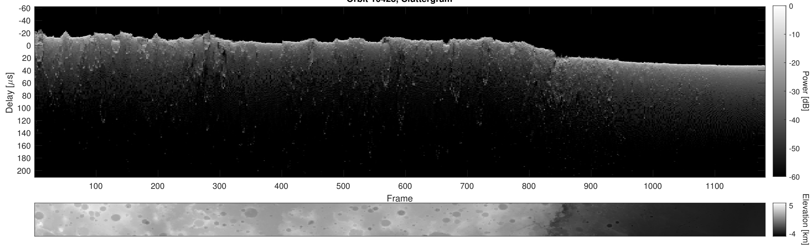
Orbit 10428, Cluttergram
