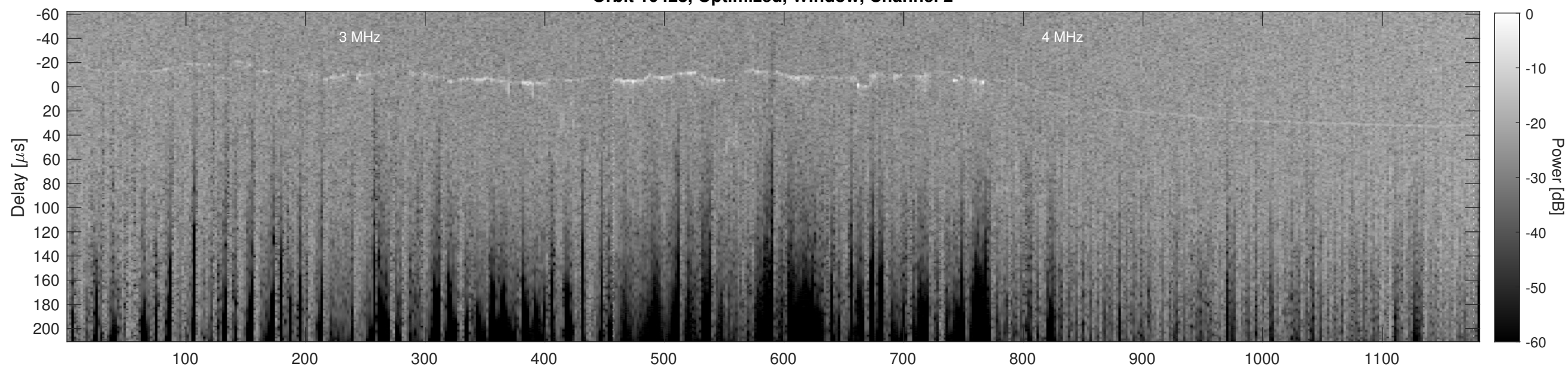
Orbit 10428, Cluttergram
