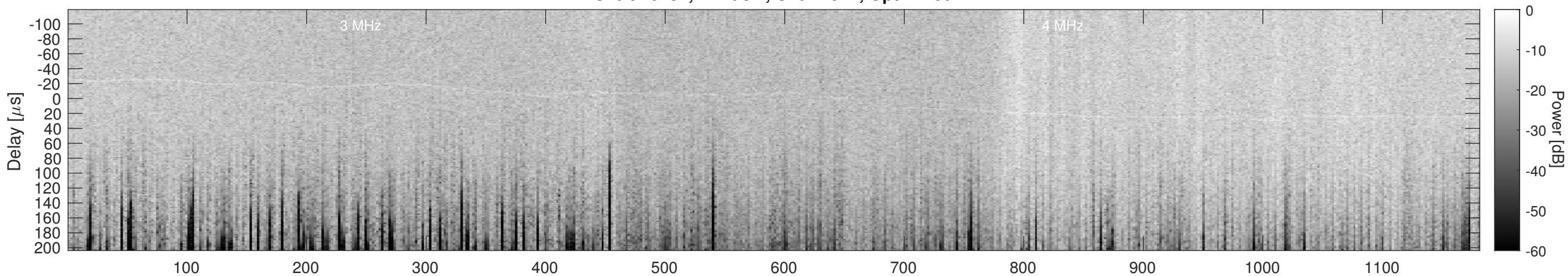
Orbit 10431, Cluttergram
