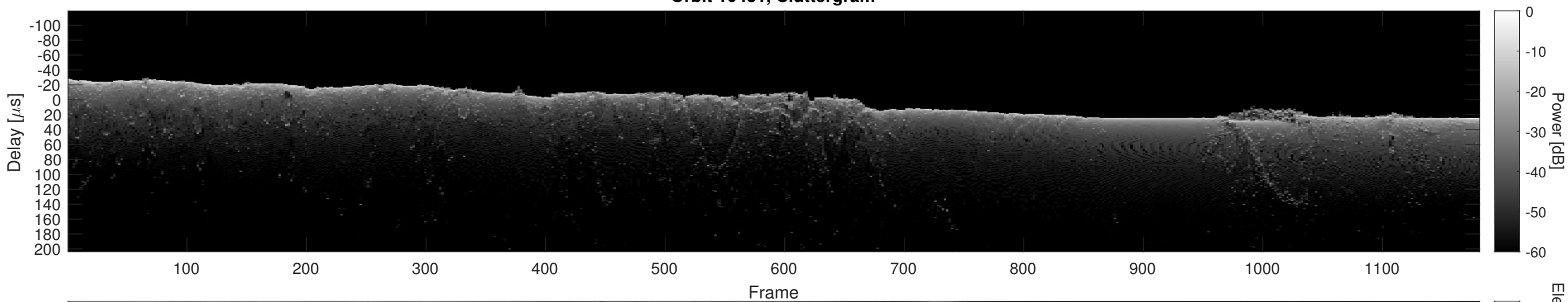
Orbit 10431, Cluttergram
