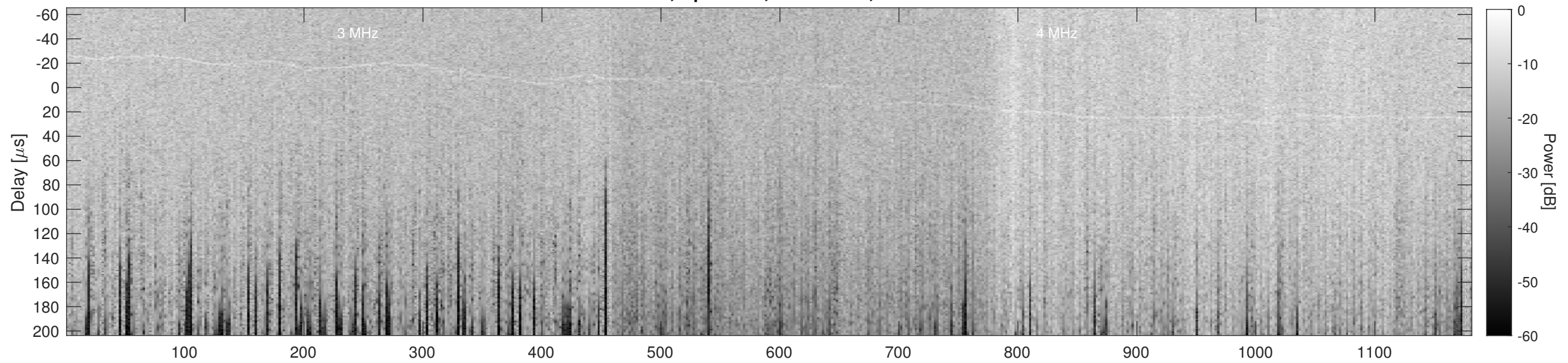
Orbit 10431, Cluttergram
