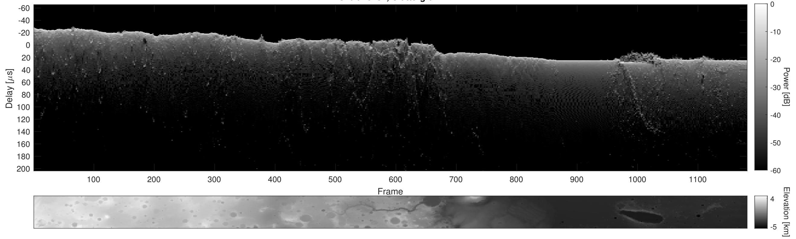
Orbit 10431, Cluttergram
