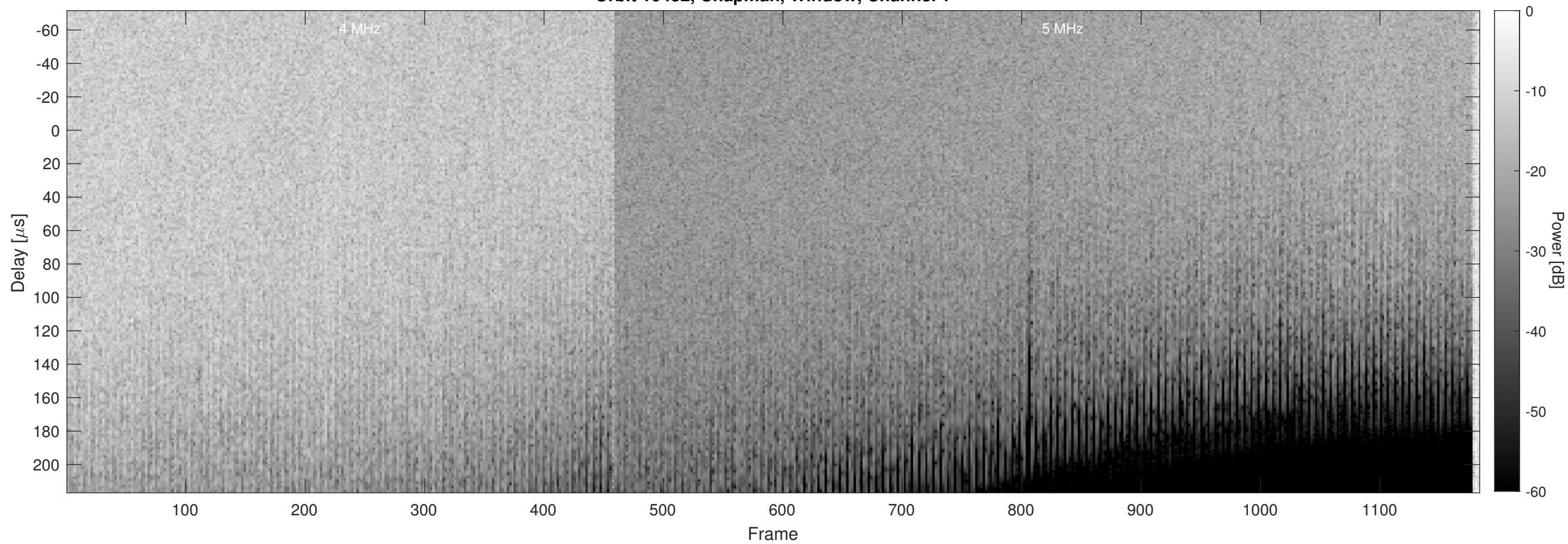
Orbit 10432, Chapman, Window, Channel 2
