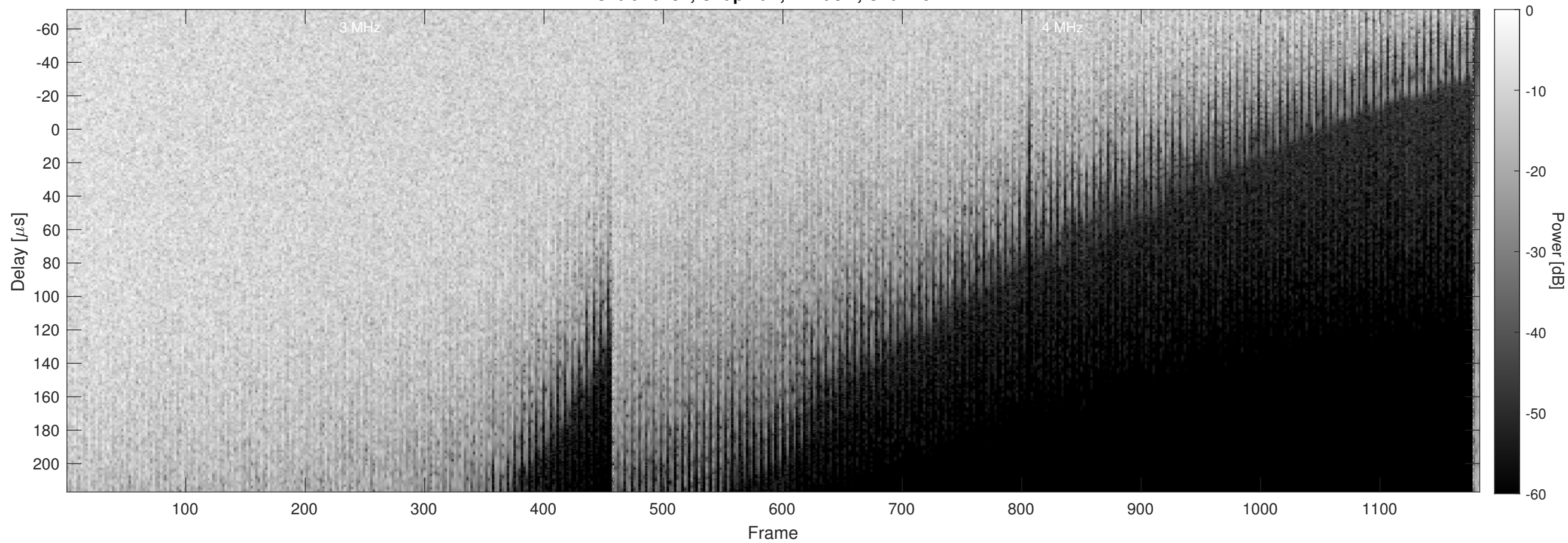
Orbit 10432, Chapman, Window, Channel 2
