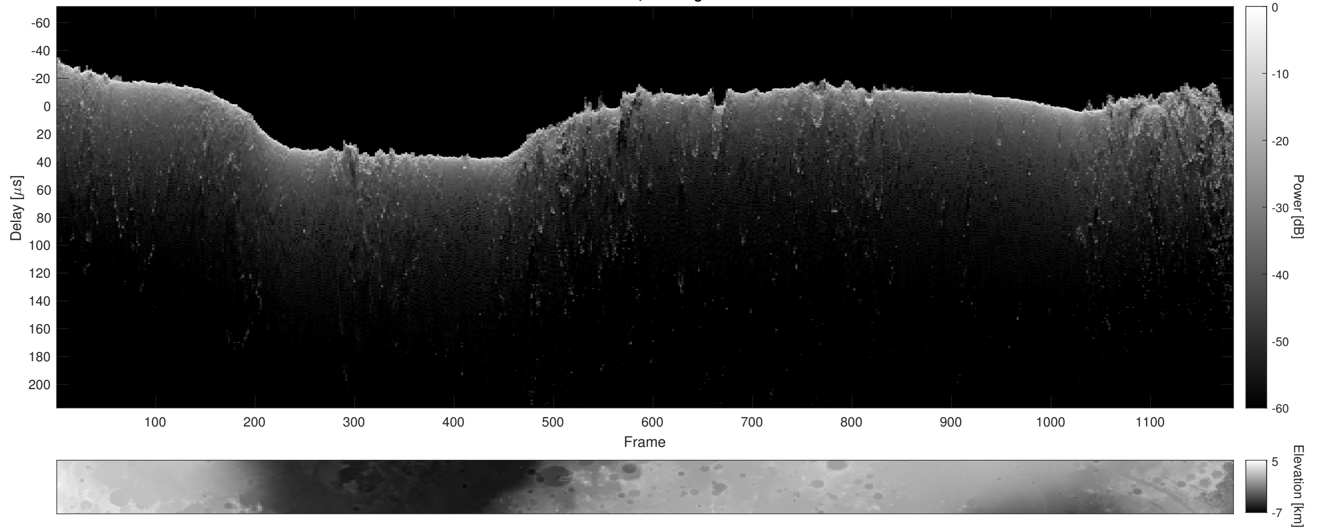
Orbit 10432, Cluttergram
