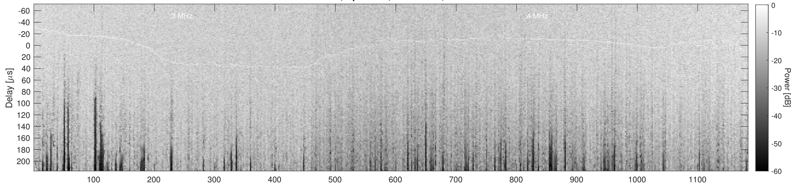
Orbit 10432, Cluttergram
