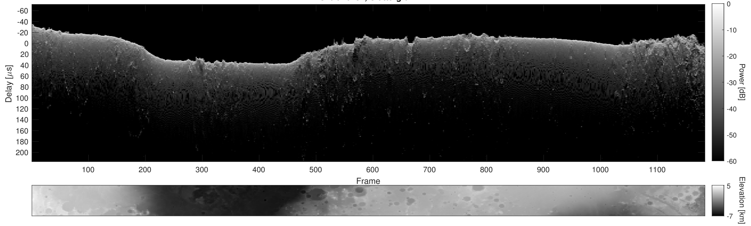
Orbit 10432, Cluttergram
