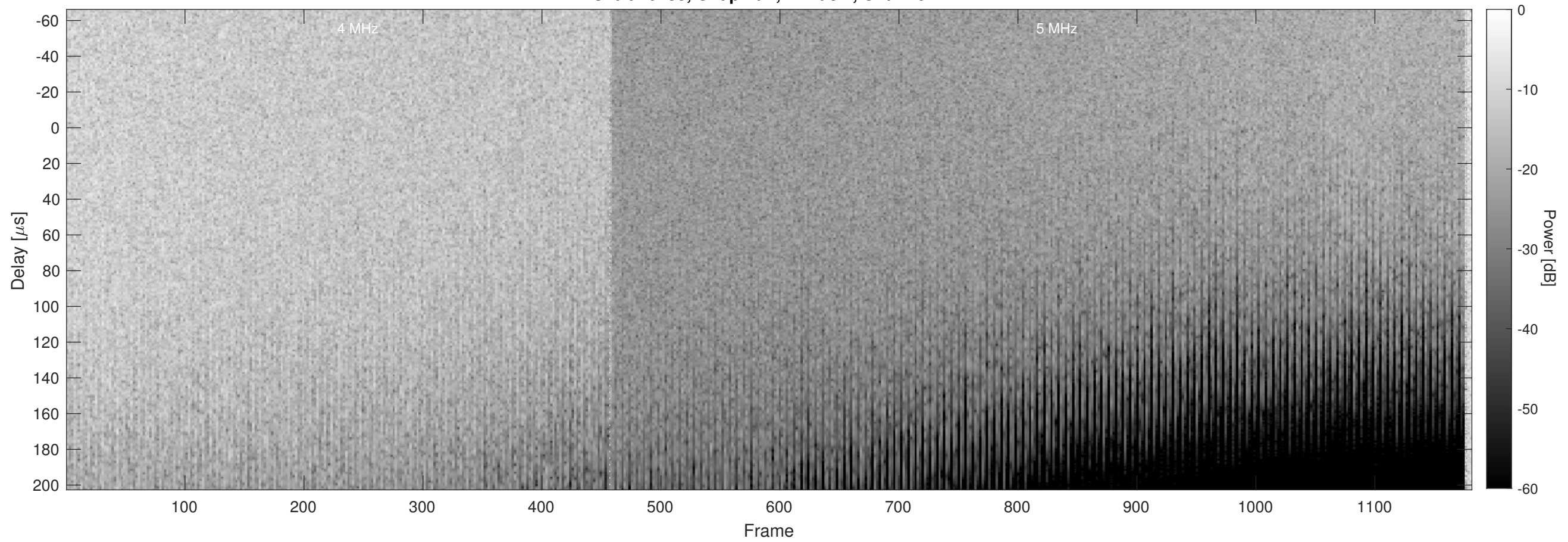
Orbit 10433, Chapman, Window, Channel 2
