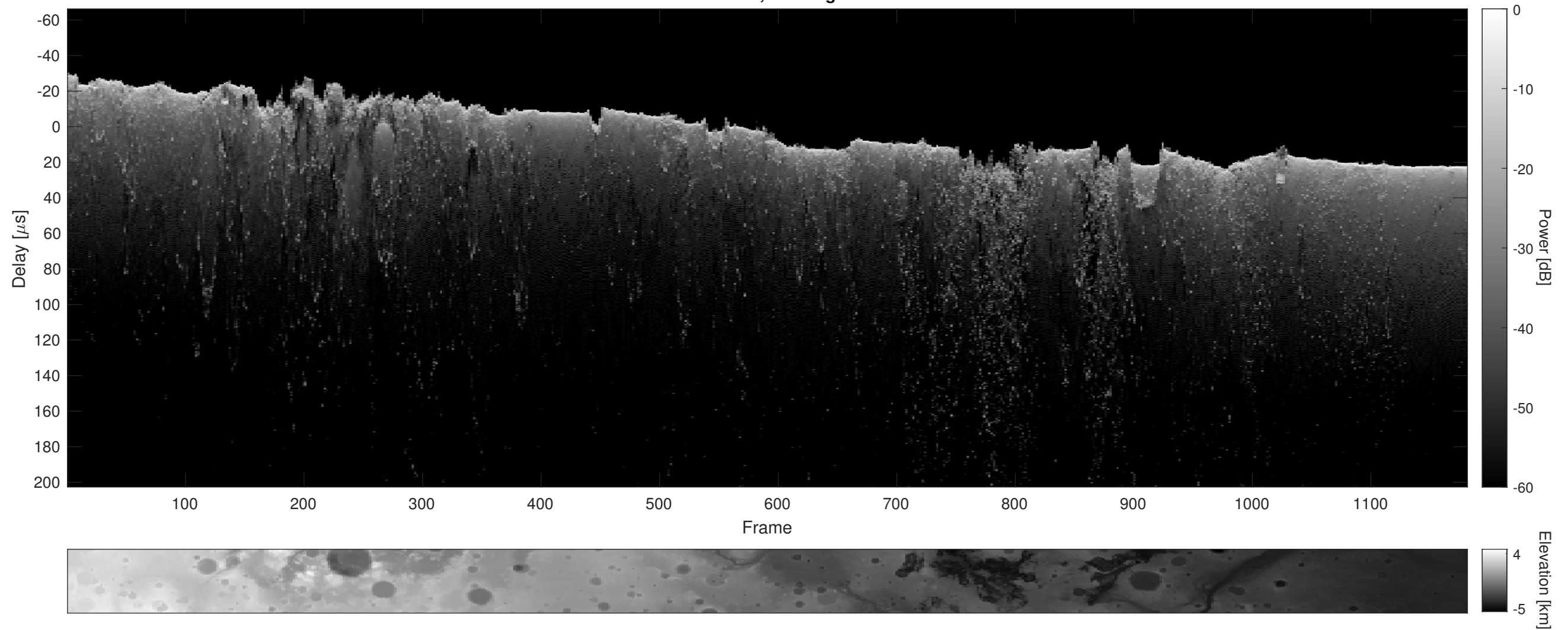
Orbit 10433, Cluttergram
