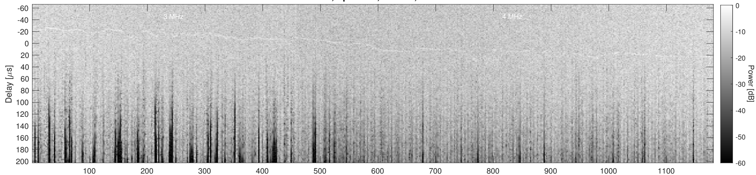
Orbit 10433, Cluttergram
