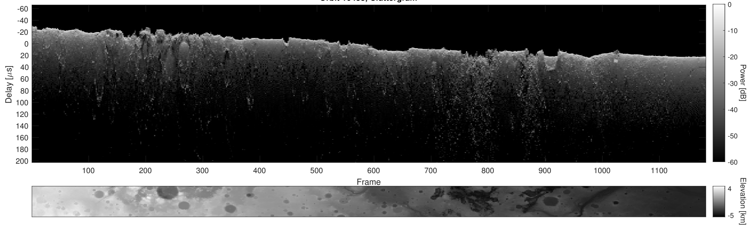
Orbit 10433, Cluttergram
