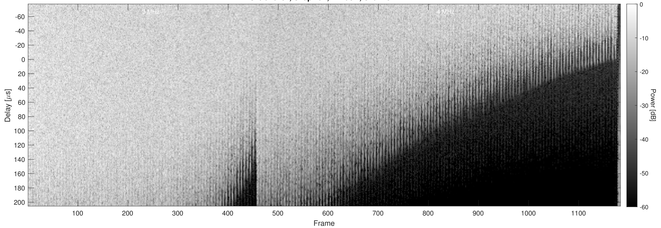
Orbit 10434, Chapman, Window, Channel 2
