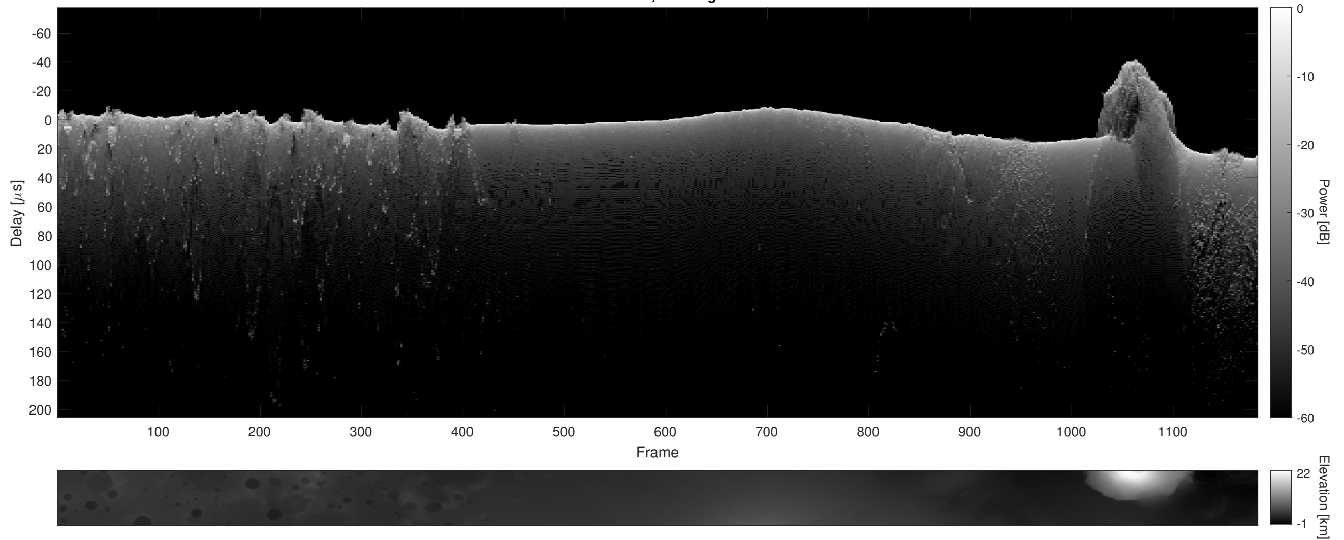
Orbit 10434, Cluttergram
