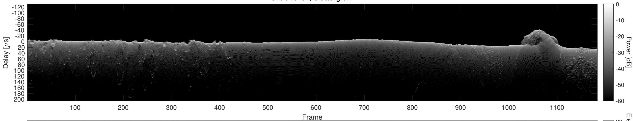
Orbit 10434, Cluttergram
