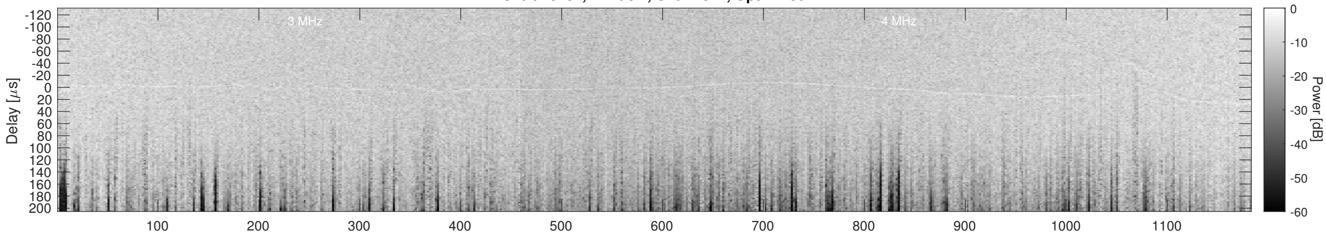
Orbit 10434, Cluttergram
