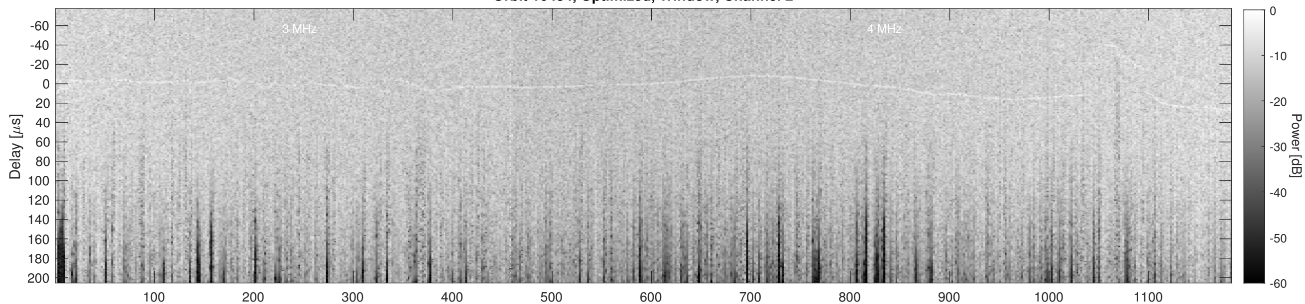
Orbit 10434, Cluttergram
