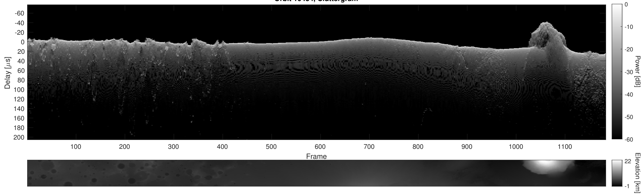
Orbit 10434, Cluttergram
