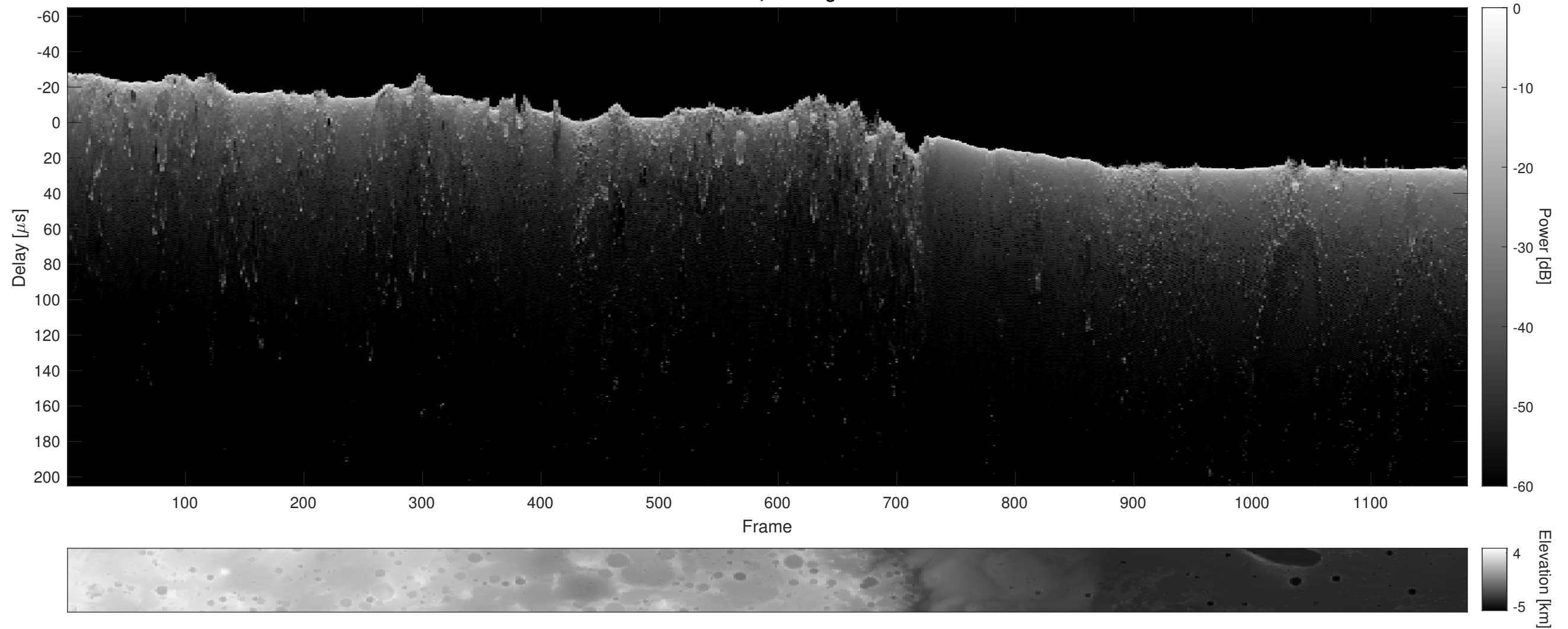
Orbit 10438, Cluttergram
