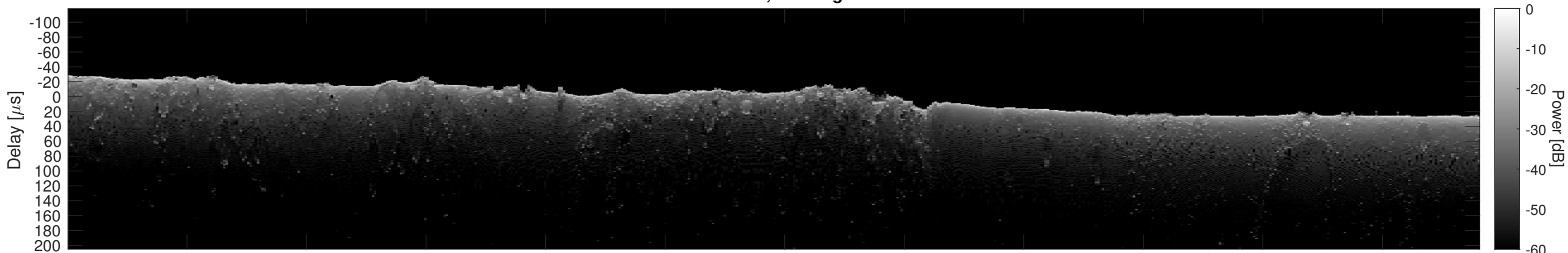
Orbit 10438, Cluttergram
