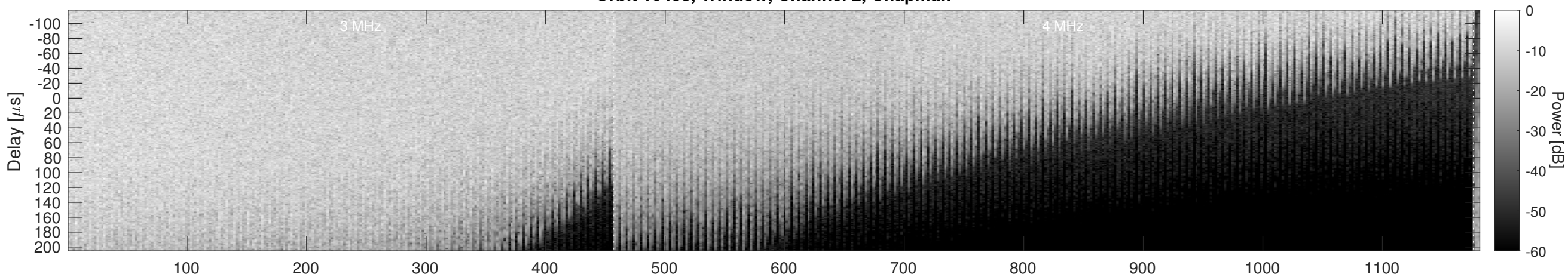
Orbit 10438, Window, Channel 2, Optimized
