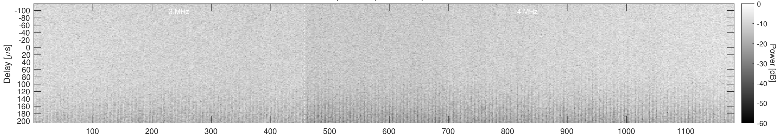
Orbit 10438, Window, Channel 2, Chapman
