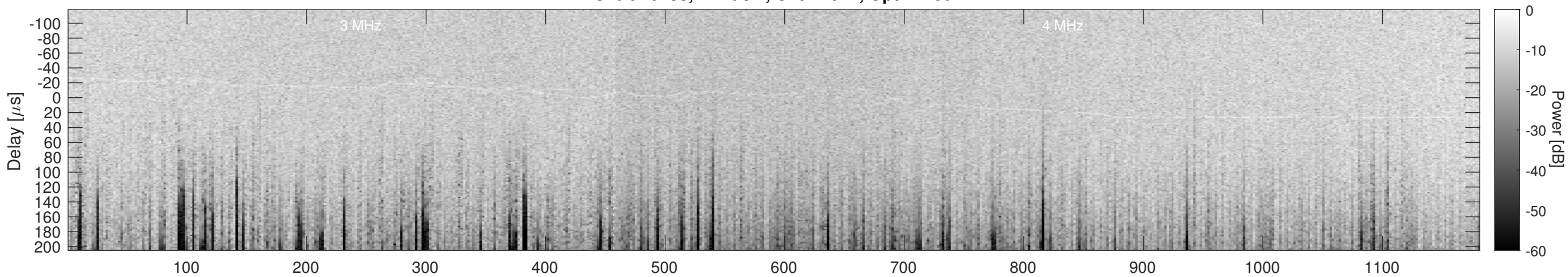
Orbit 10438, Cluttergram
