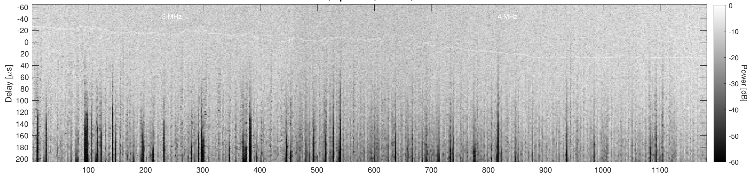
Orbit 10438, Cluttergram
