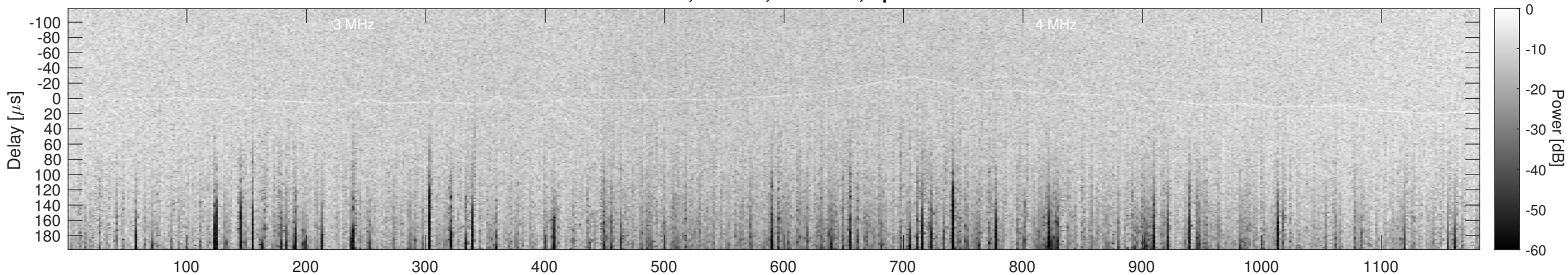
Orbit 10441, Cluttergram
