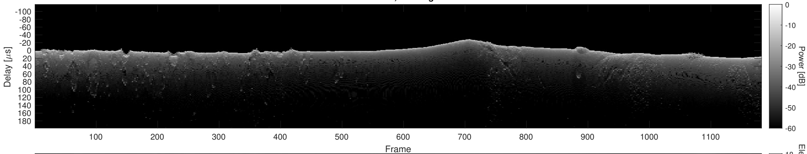
Orbit 10441, Cluttergram
