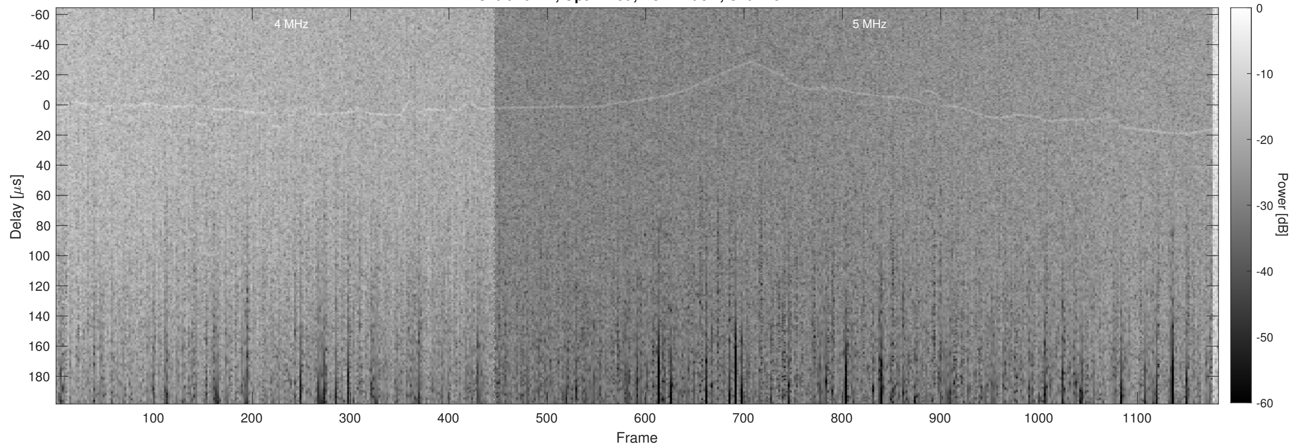
Orbit 10441, Optimized, No Window, Channel 2
