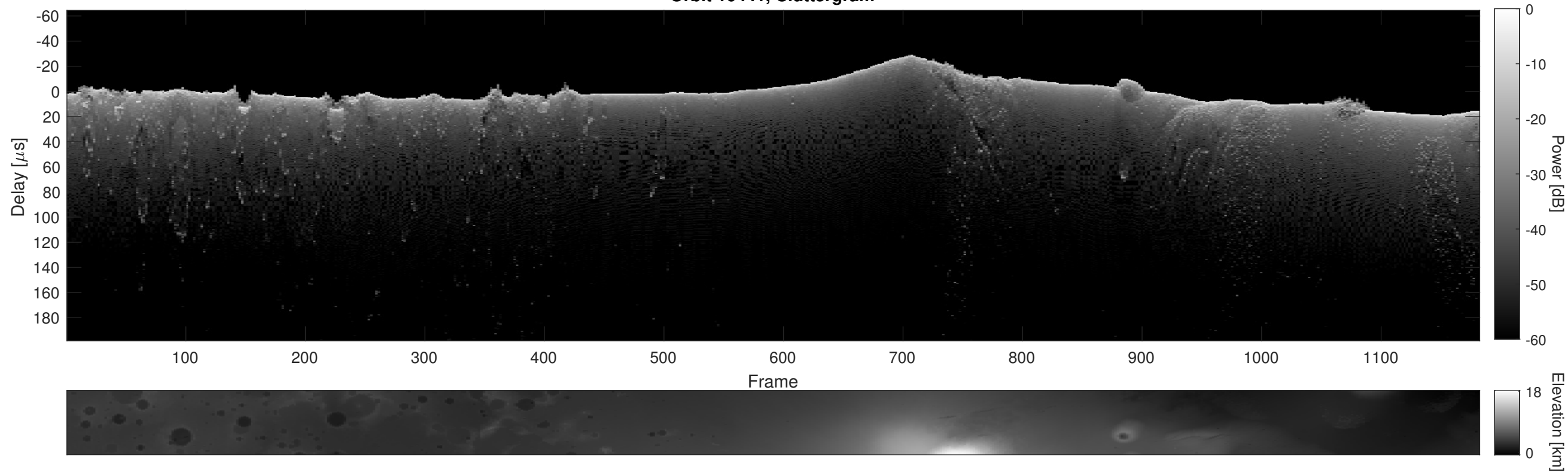
Orbit 10441, Cluttergram
