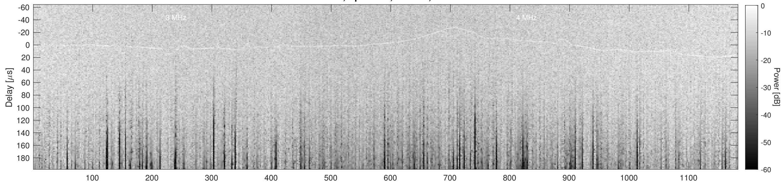
Orbit 10441, Cluttergram
