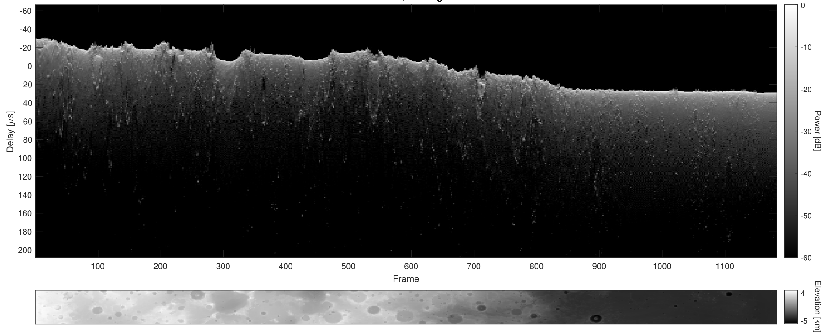
Orbit 10459, Cluttergram
