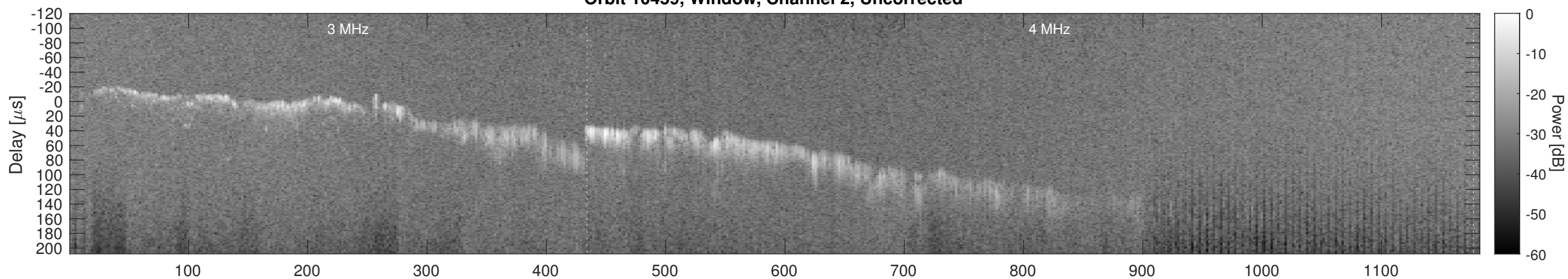
Orbit 10459, Window, Channel 2, Chapman
