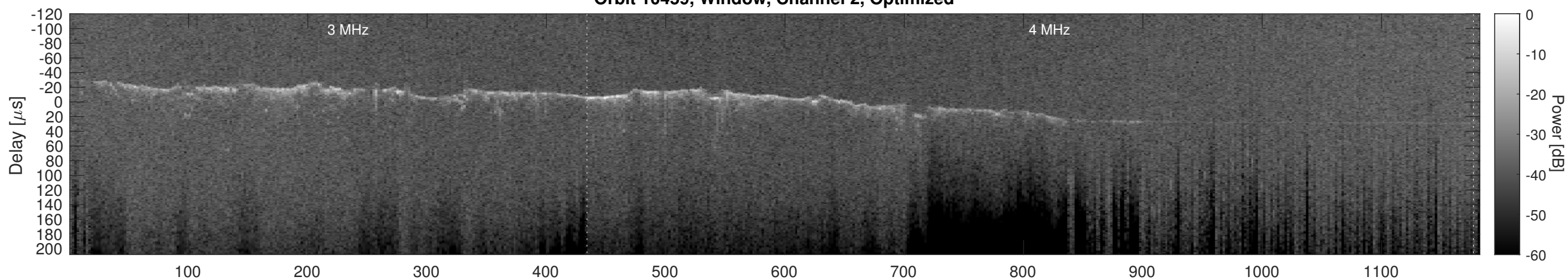
Orbit 10459, Cluttergram
