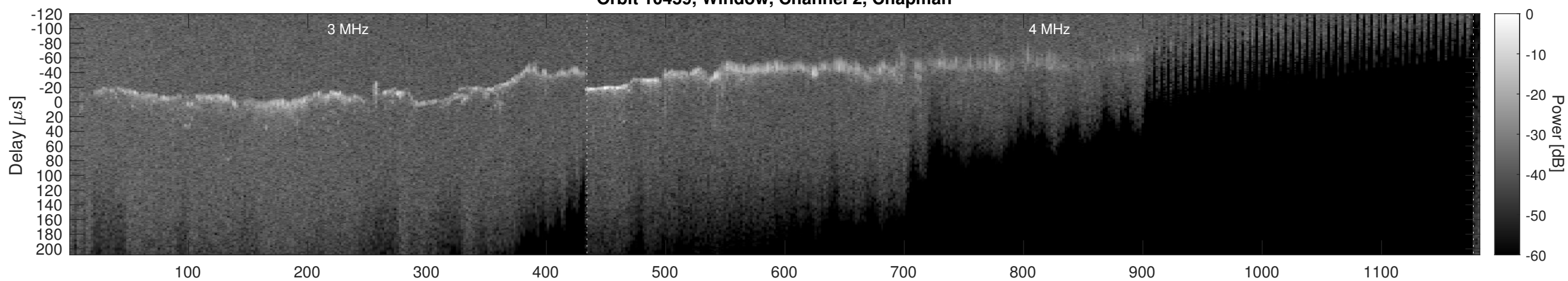
Orbit 10459, Window, Channel 2, Optimized
