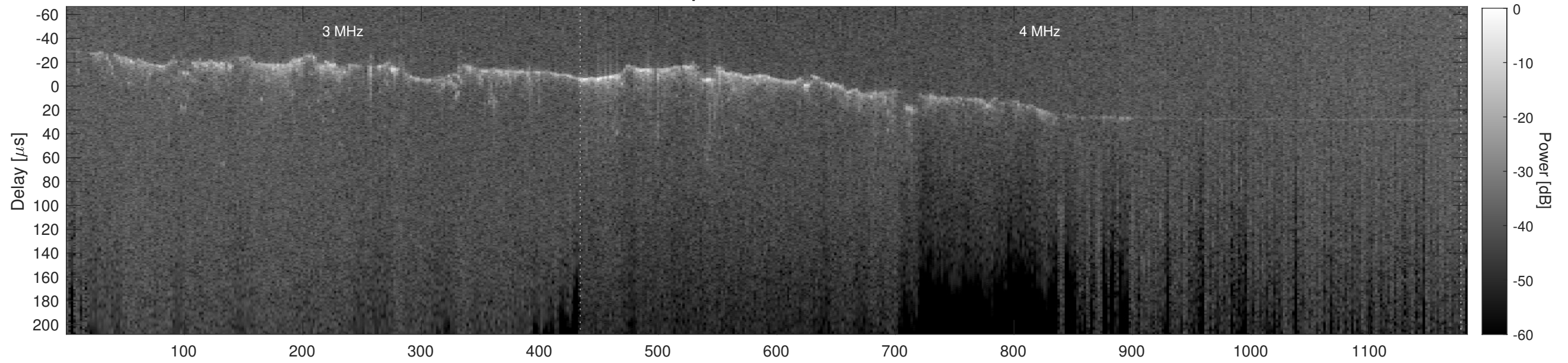
Orbit 10459, Cluttergram
