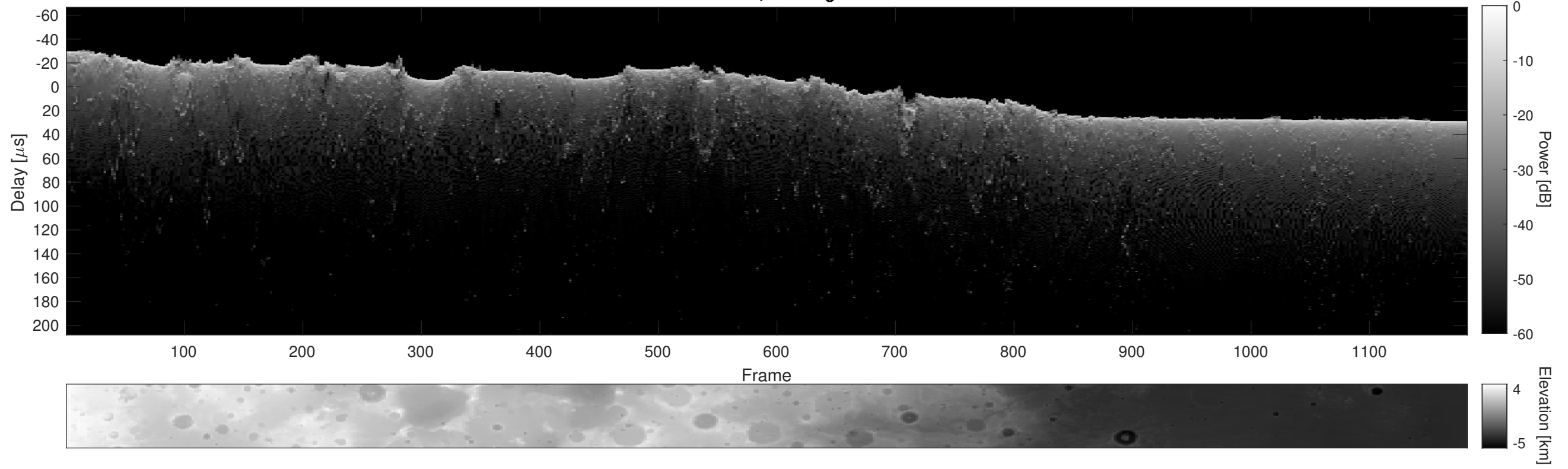
Orbit 10459, Cluttergram
