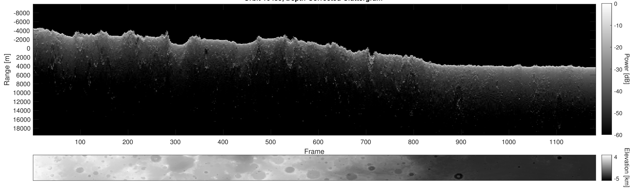
Orbit 10459, Depth-Corrected Cluttergram
