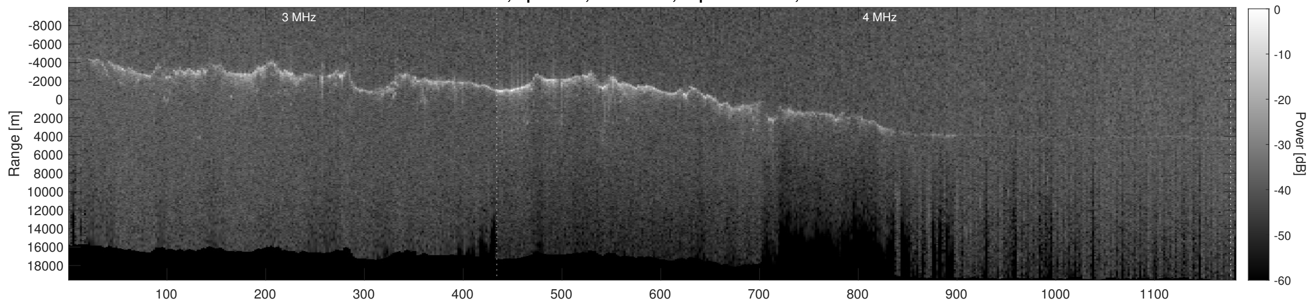
Orbit 10459, Depth-Corrected Cluttergram
