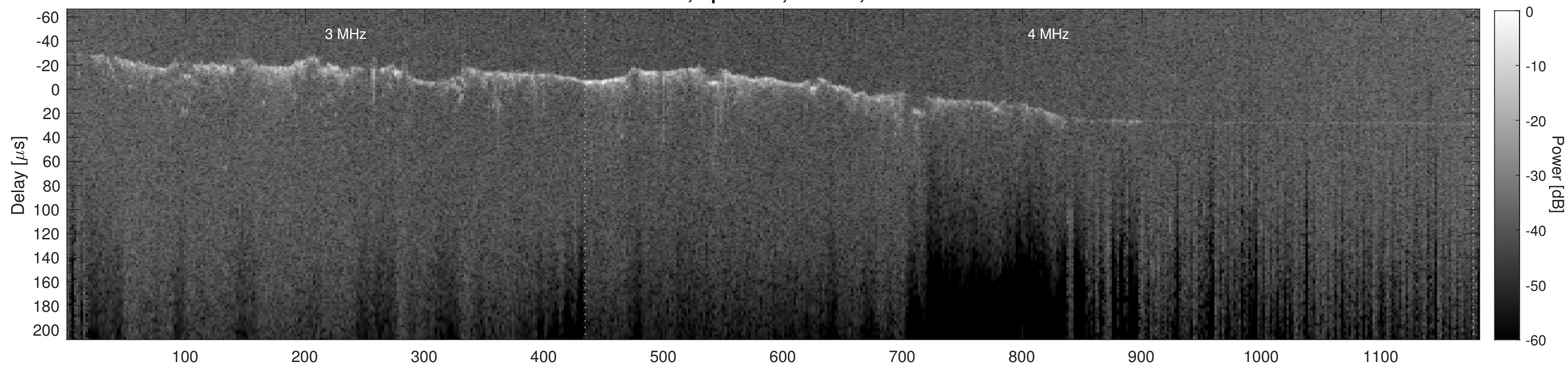
Orbit 10459, Cluttergram
