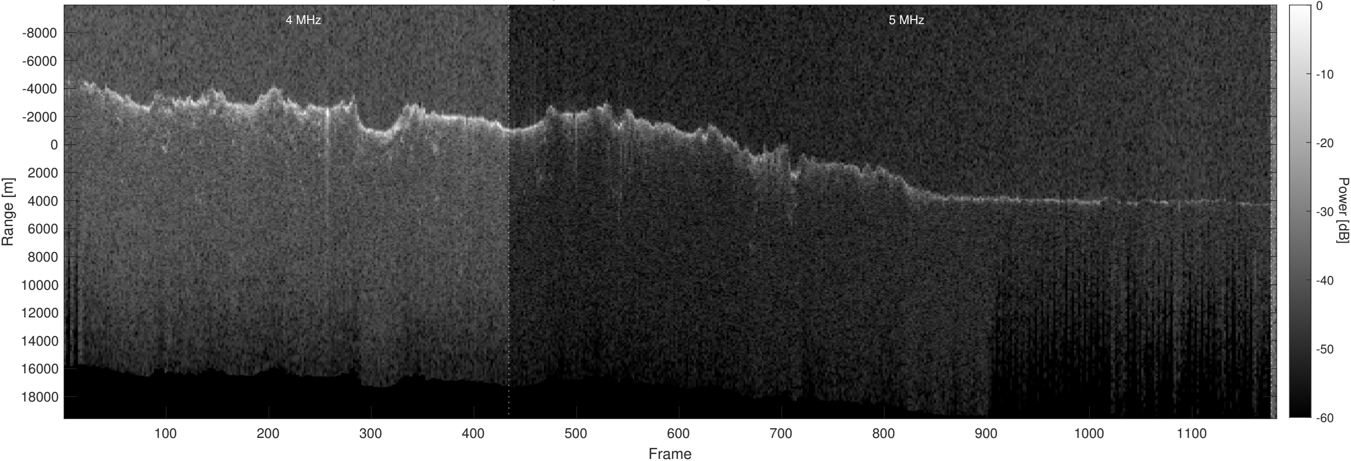
Orbit 10459, Optimized, Window, Depth-Corrected, Channel 2
