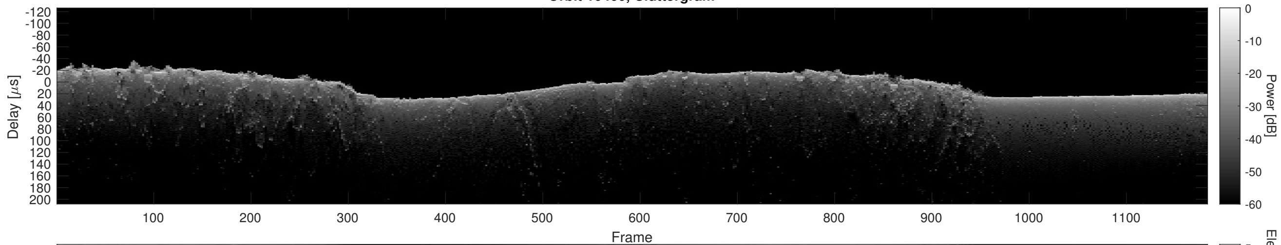
Orbit 10460, Cluttergram
