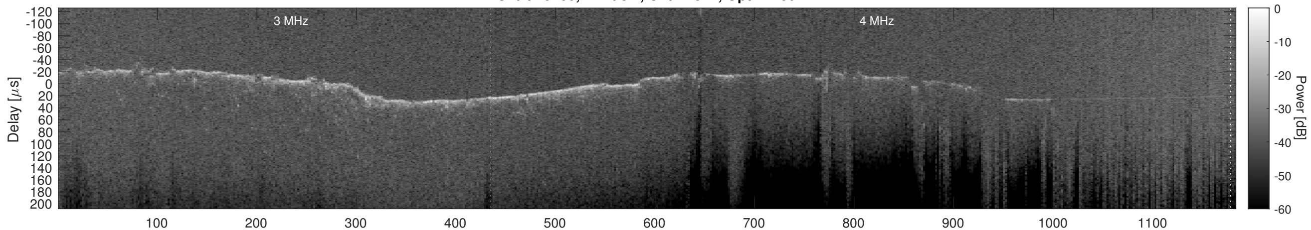
Orbit 10460, Cluttergram
