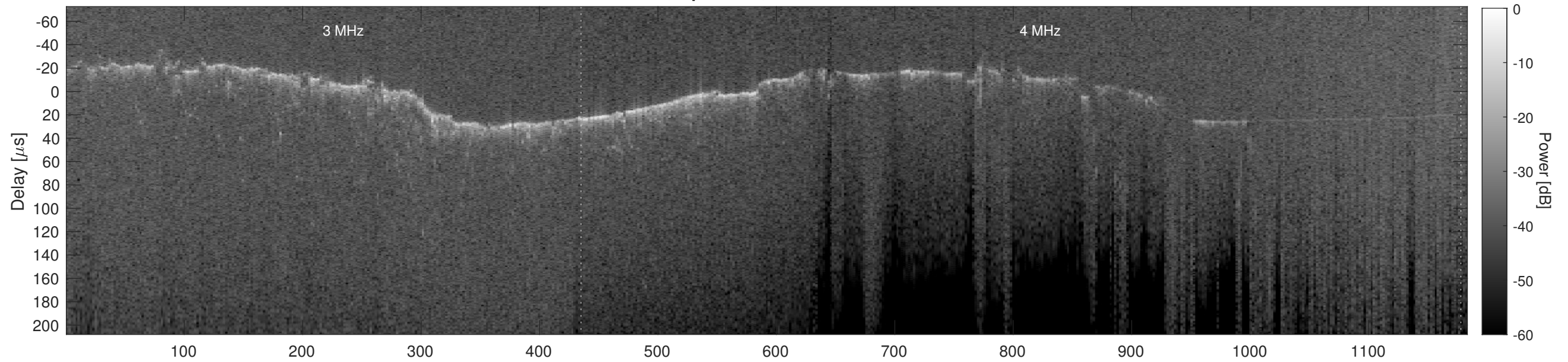
Orbit 10460, Cluttergram
