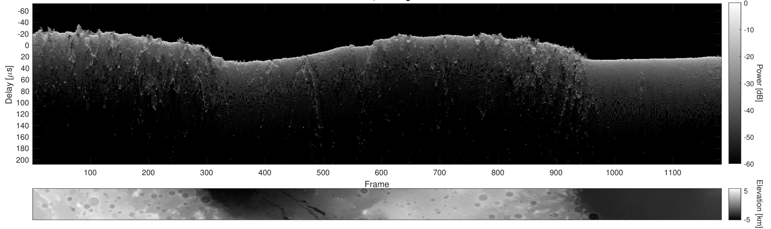
Orbit 10460, Cluttergram
