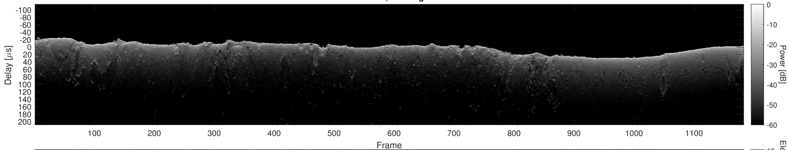
Orbit 10463, Cluttergram
