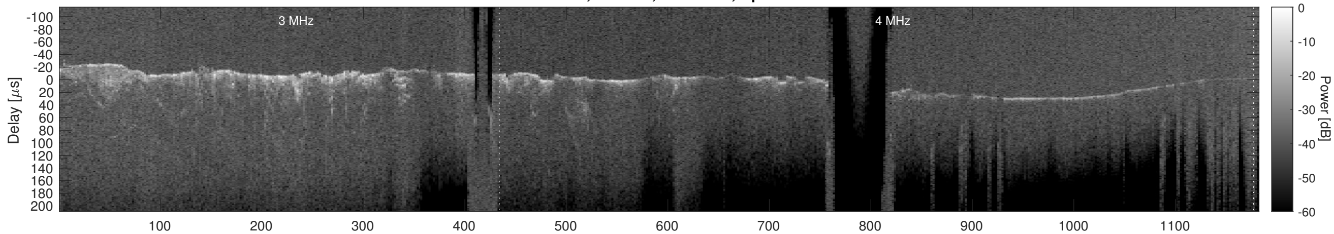
Orbit 10463, Cluttergram
