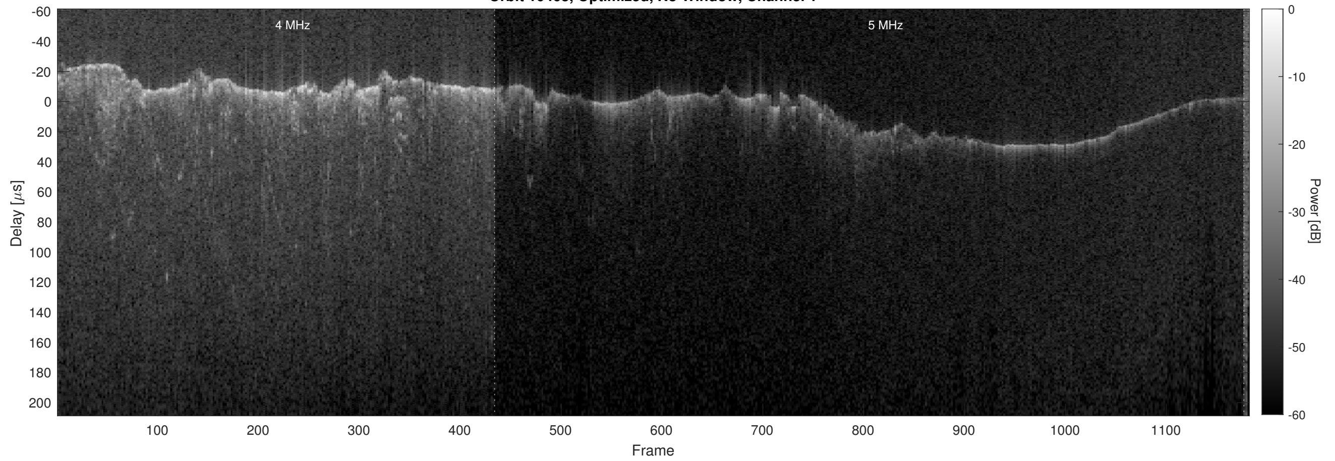
Orbit 10463, Optimized, No Window, Channel 2
