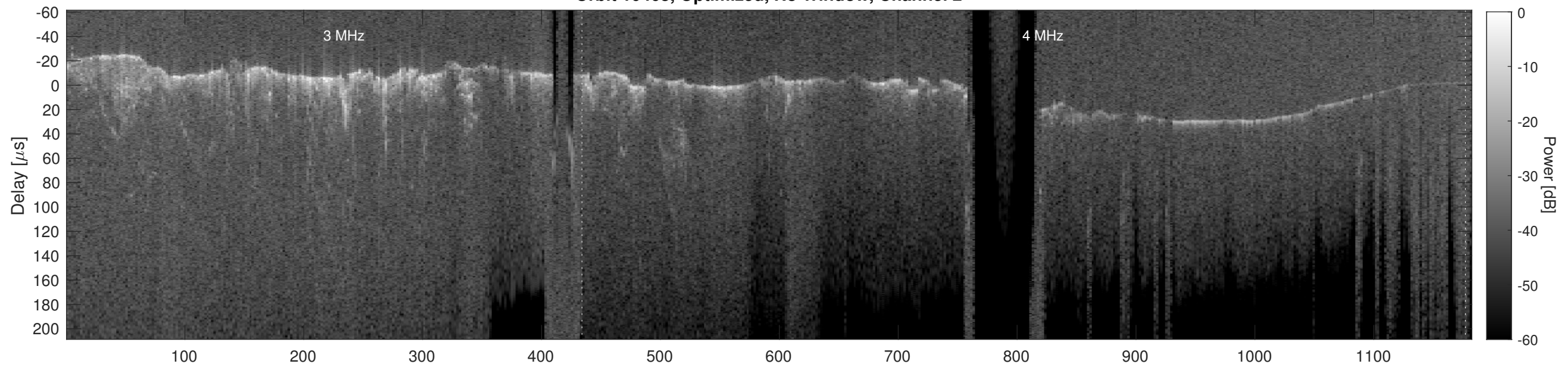
Orbit 10463, Cluttergram
