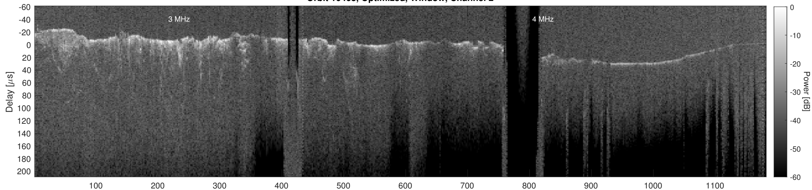
Orbit 10463, Cluttergram
