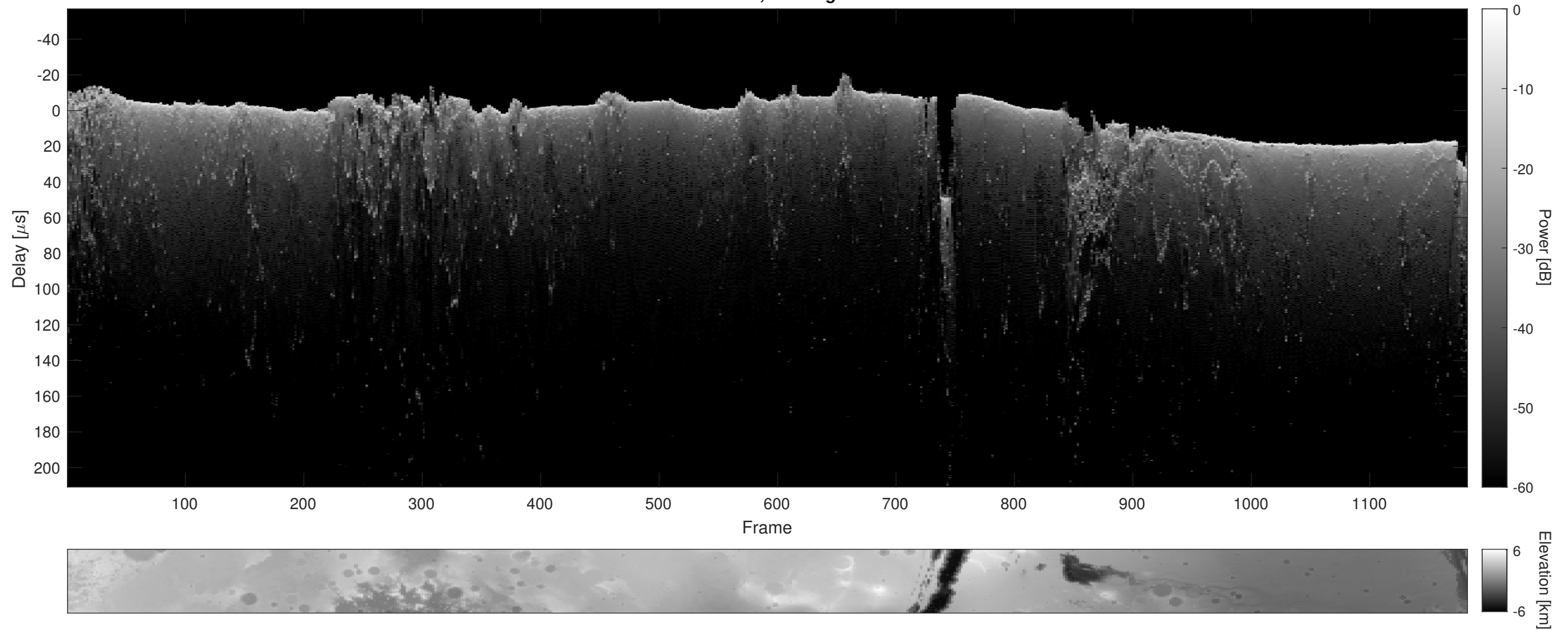
Orbit 10465, Cluttergram
