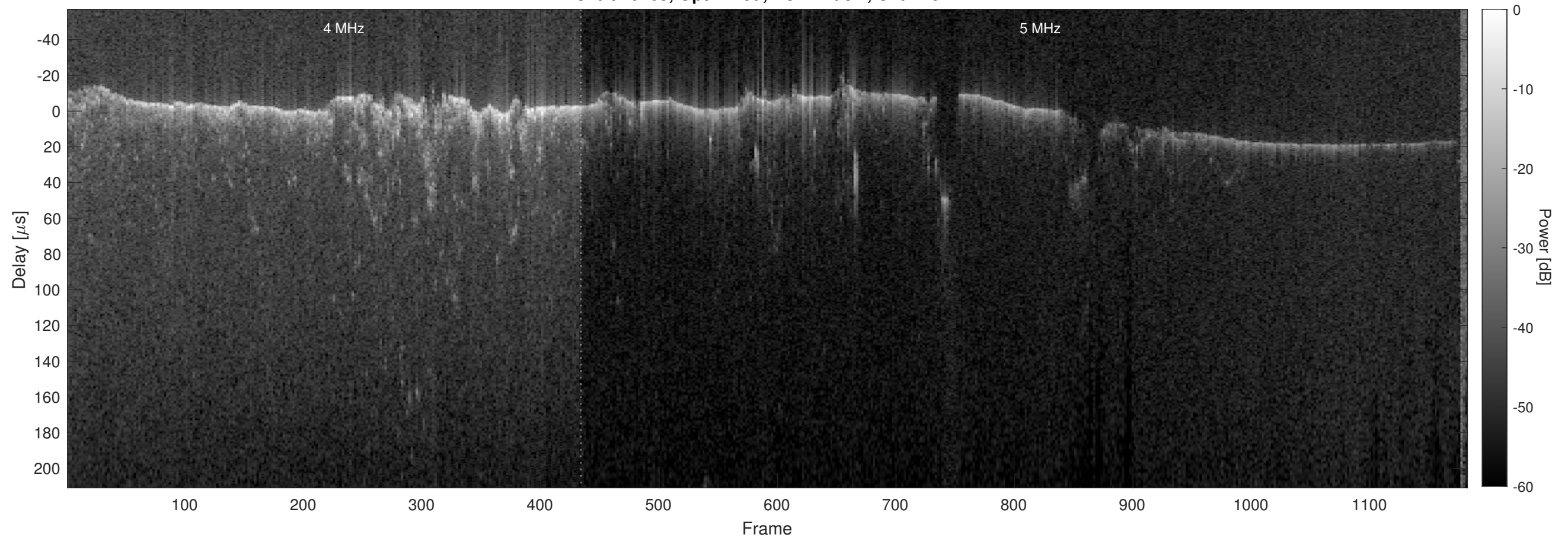
Orbit 10465, Optimized, No Window, Channel 2
