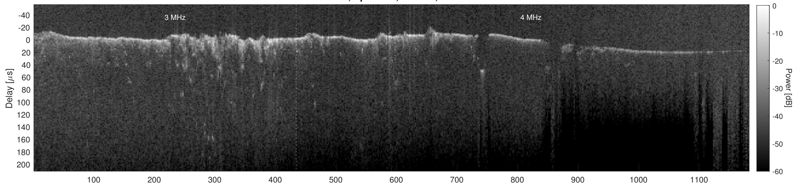
Orbit 10465, Cluttergram
