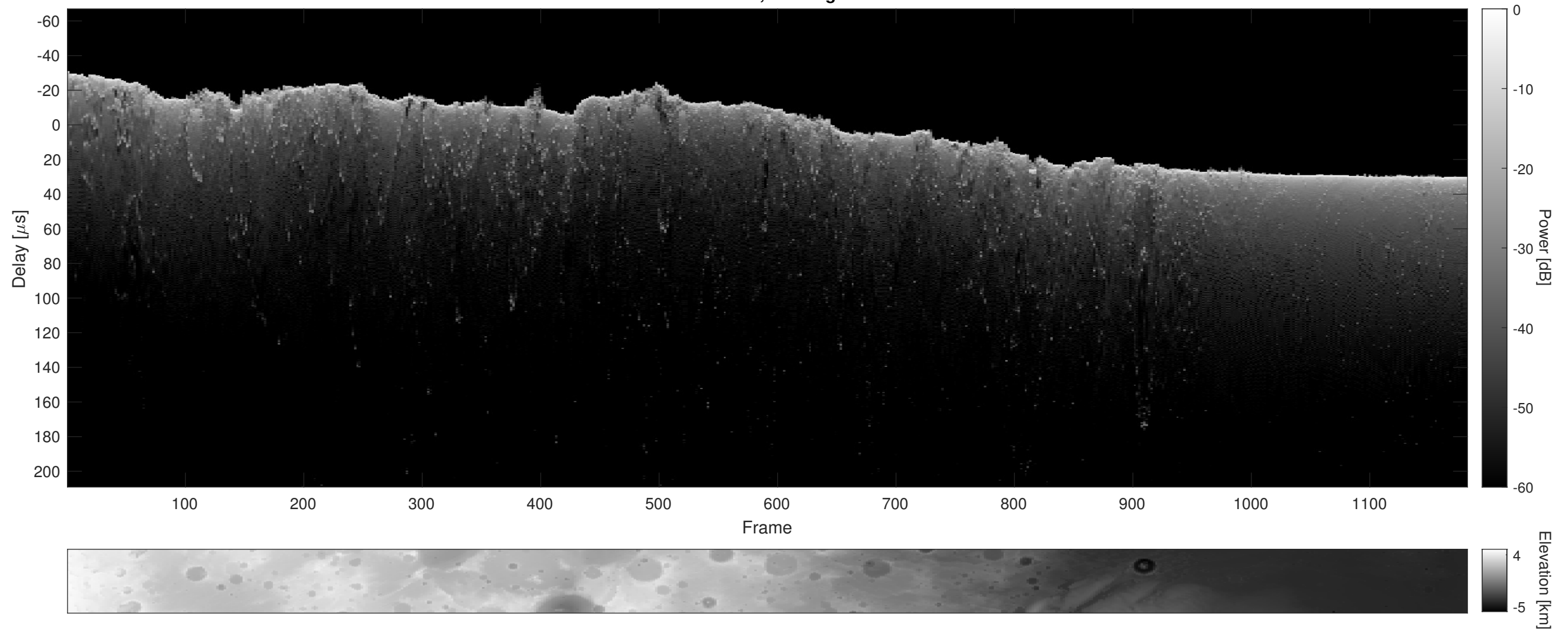
Orbit 10466, Cluttergram
