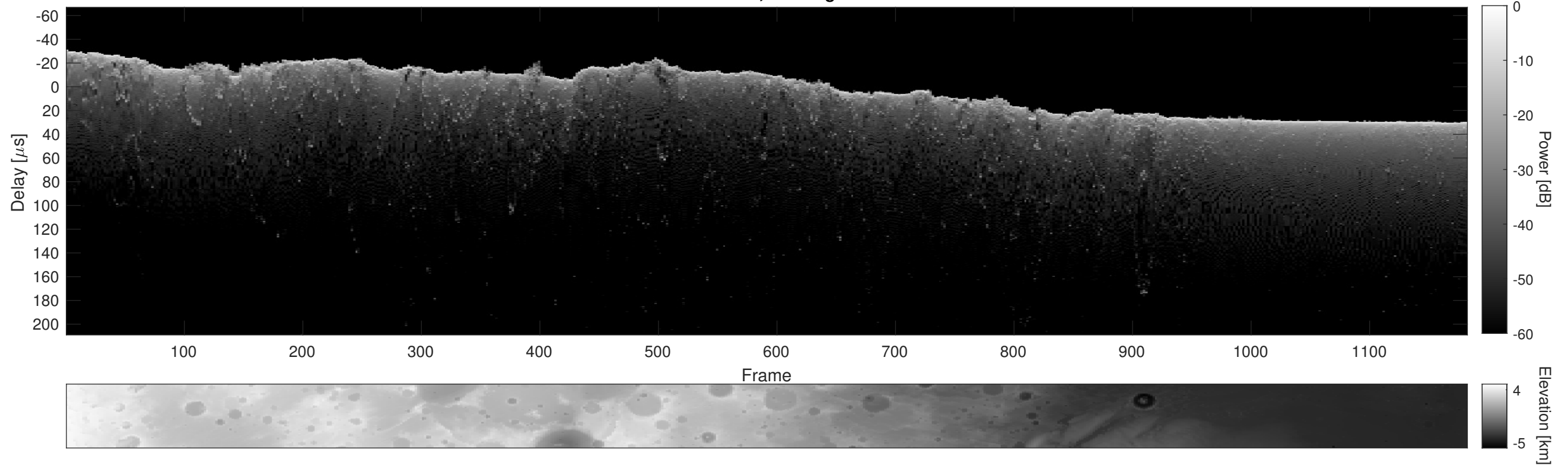
Orbit 10466, Cluttergram
