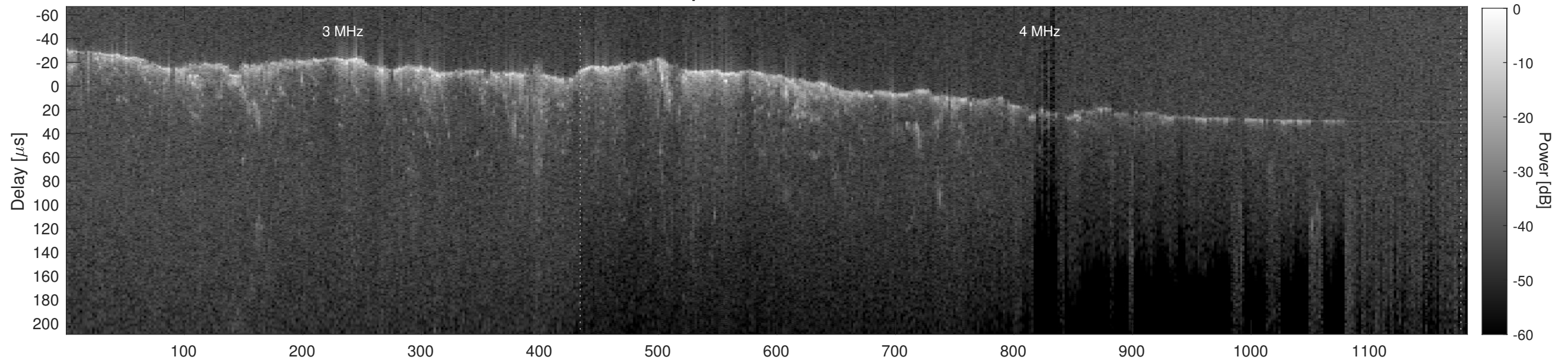
Orbit 10466, Cluttergram
