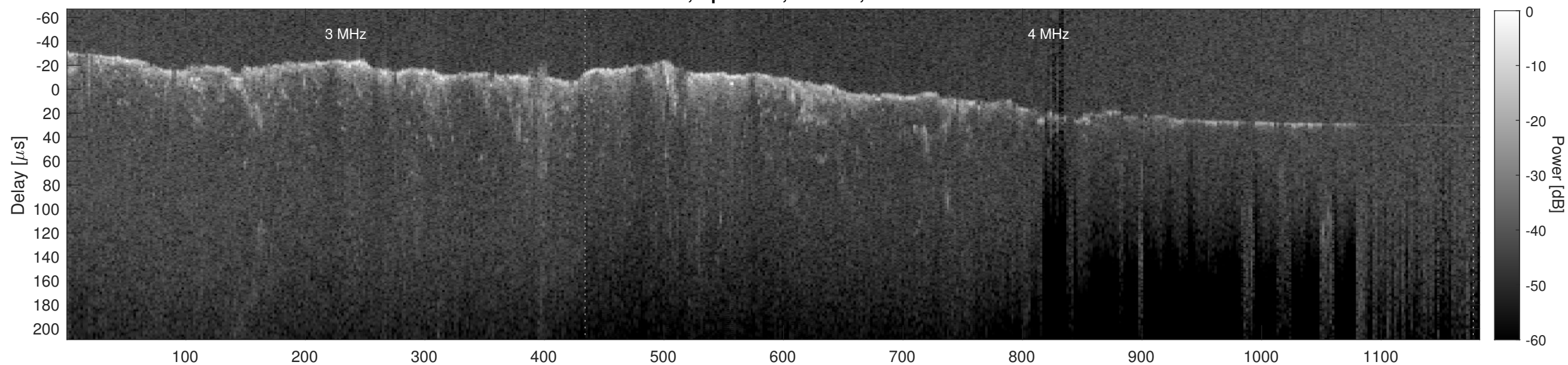
Orbit 10466, Cluttergram
