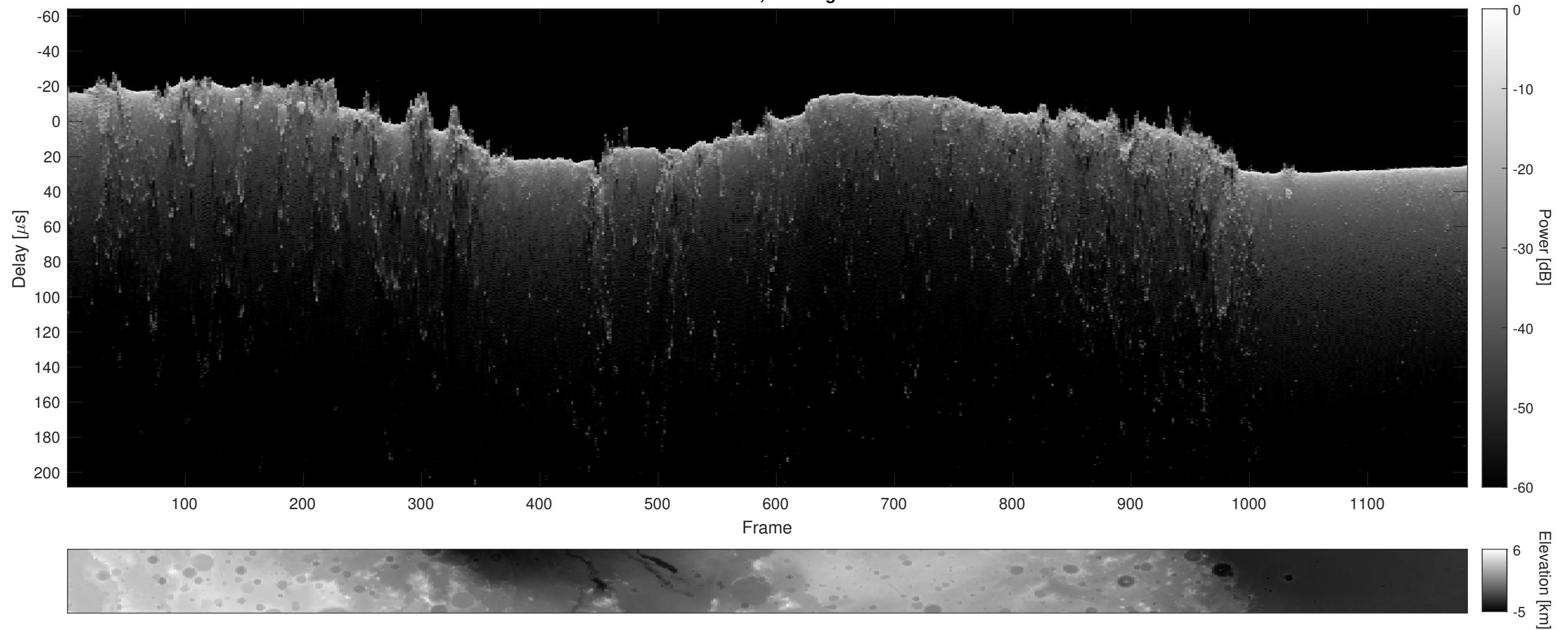
Orbit 10467, Cluttergram
