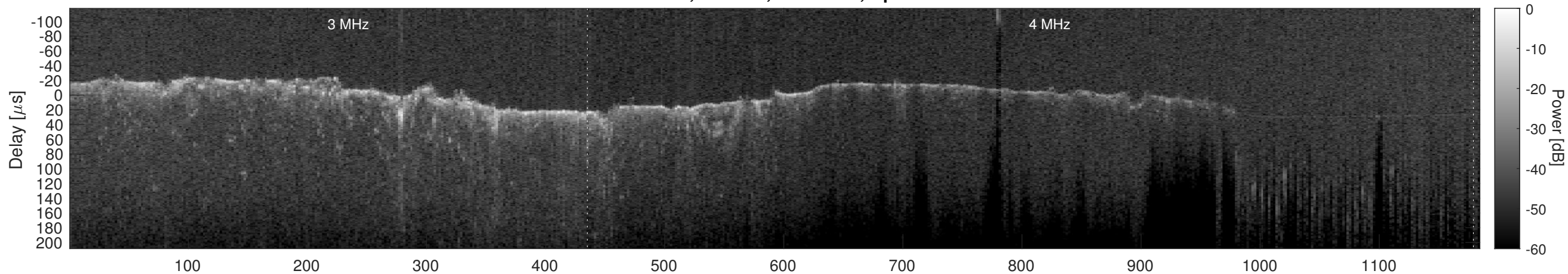
Orbit 10467, Cluttergram
